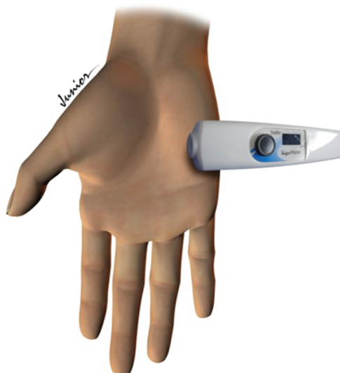
Figure 1 – Measurement of the intensity of palmar sweating.
