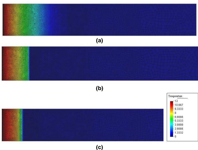
Figure 8. Tissue temperature field at time instant t = 15.25 s: (a) \tau_r = 0 s considering the ExGA-Stehfest scheme; (b) \tau_r = 10 s considering the ExGA-Stehfest linear \theta scheme with \theta = 1.2 ; (c) \tau_r = 20 s considering the ExGA-Stehfest linear \theta scheme with \theta = 1.2 .
