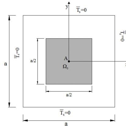
Figure 9. Geometry and boundary conditions of the square biological tissue body under initial temperature field over the domain \Omega_0 .
