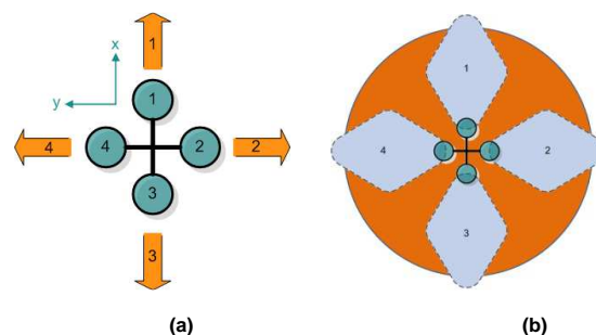
Figure 10. (a) Visualization of the 4 flight directions and (b) illustration of the 150 cm security zone around the OS4.
