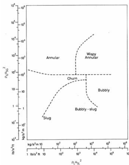
Figure 4. Hewitt and Roberts (1969) map for vertical flow.
