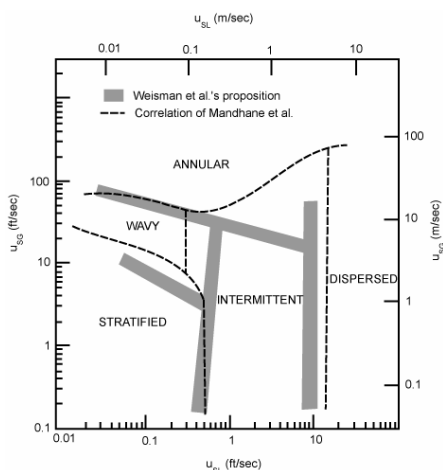
Figure 6. Weisman et al. (1979) map for horizontal flow.
