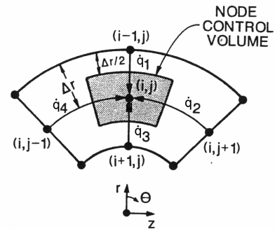
Figure 8. Finite-difference grid arrangement (Ghajar and Zurigat, 1991).
