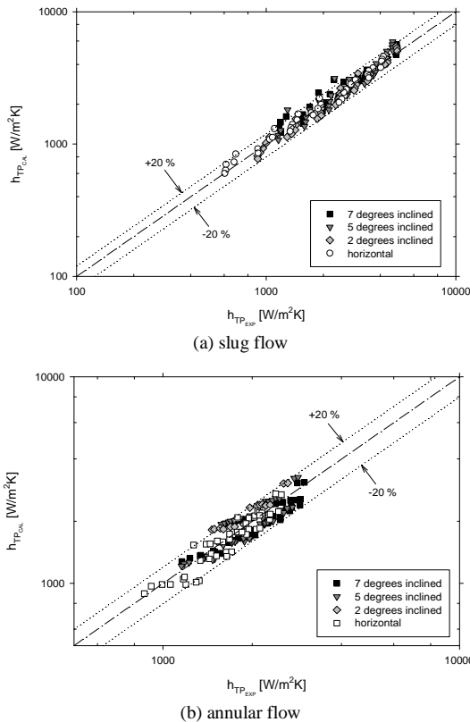
Figure 28. Comparison of the predictions of the recommended heat transfer correlation, eq.(65),with the horizontal and inclined slug and annular air-water flow experimental data.
