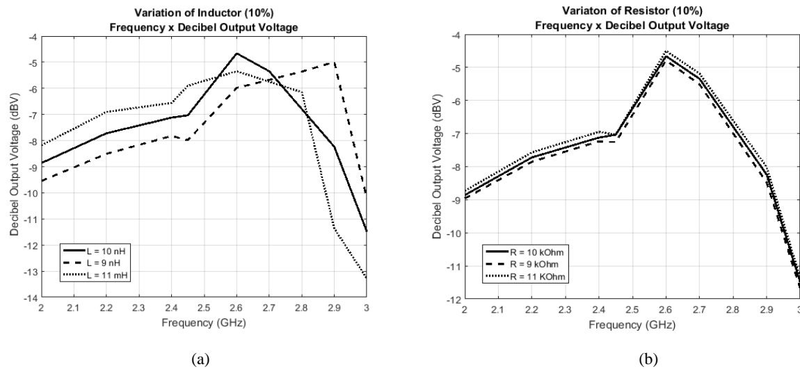
Fig. 18. Accuracy of Components: (a) Inductor and (b) Resistor.
