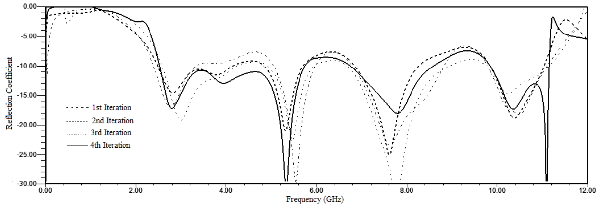
Fig. 3. Effect on the return loss characteristics due to increase in iterations
