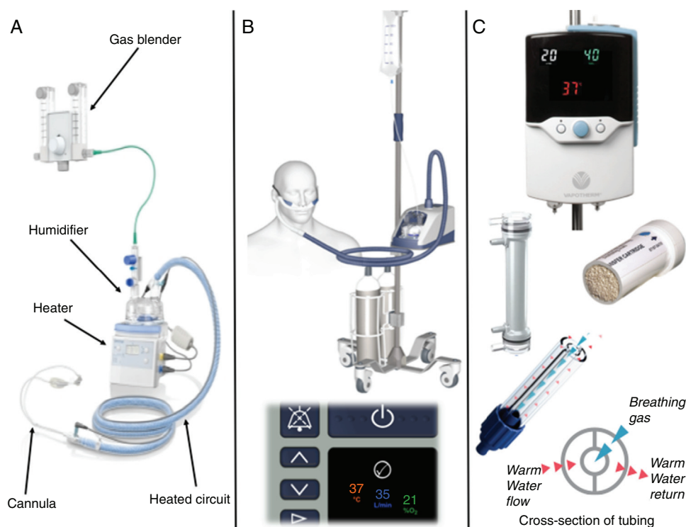
Figure 1 Examples of commercially available devices to deliver high-flow nasal cannula (HFNC) support. Panel A: HFNC system assembled from commonly available components, including a blender, heater/humidifier, heated circuit, and cannula. Panel B: the Airvo 2 HFNC system shown here as a mobile unit with air and oxygen cylinders (top), and a close up of the digital console indicating the set temperature, flow and oxygen concentration of the inspired gas (bottom). Panel C: the Precision Flow HFNC system (top), the internal humidification cartridge and a cutout showing the hollow-fiber configuration (middle), and a cutout of the circuit with a diagram of the warm water insulation system (bottom). Images courtesy of Fisher & Paykel Healthcare Limited (A and B) and Vapotherm Inc (C).
