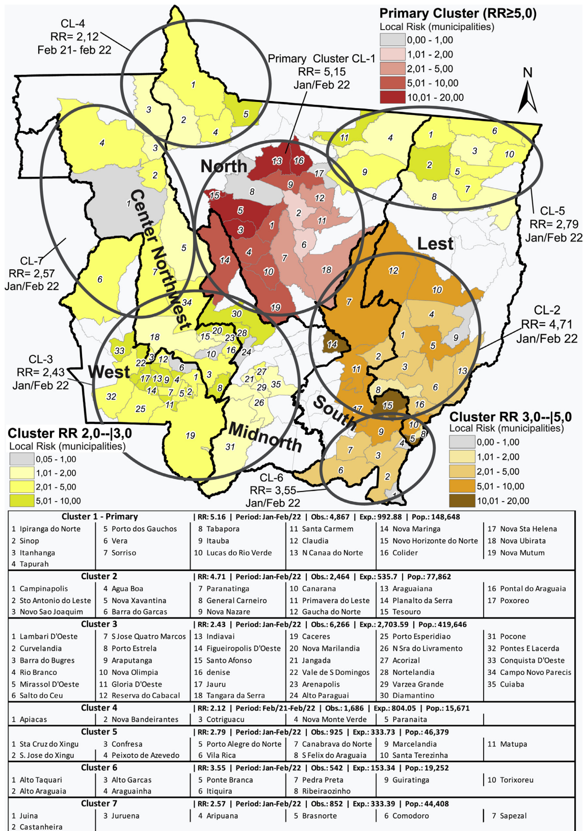
Figure 2 Space-time clusters at high risk for COVID-19 among children and adolescents aged from 0 to 19 years old, Mato Grosso, Brazil (2020–2022). Source: Data from the INDICASUS Information System; Mato Grosso (SES/MT).
