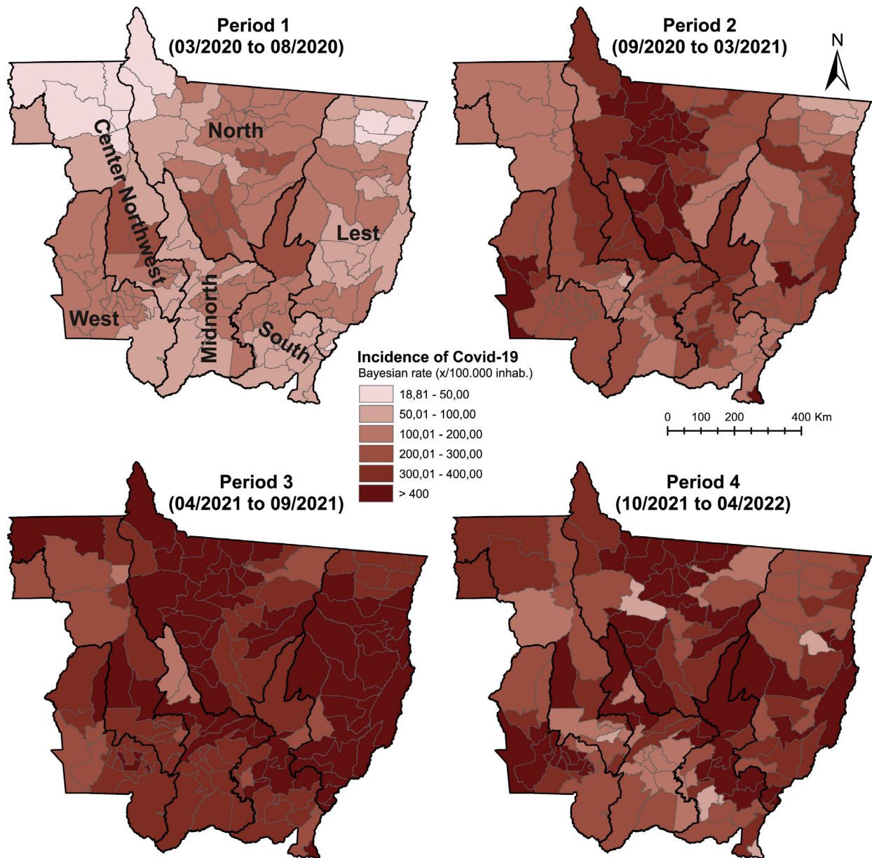
Figure 1 Space-time distribution of the COVID-19/100,000 inhabitants Bayesian incidence rates among children and adolescents aged from 0 to 19 years old, Mato Grosso, Brazil (2020–2022). Source: Data from the INDICASUS Information System; Mato Grosso (SES/MT).
