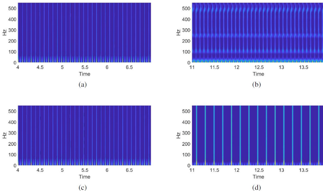
Figure 7: CWT of the signals at resonance: (a) Hertz model, (b) Experimental signal, (c) Viscoelastic model and (d) Hard collision model.
