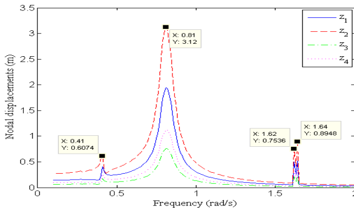
Fig. 8(a): Exact FDR for inextensible cables under general harmonic loading.
