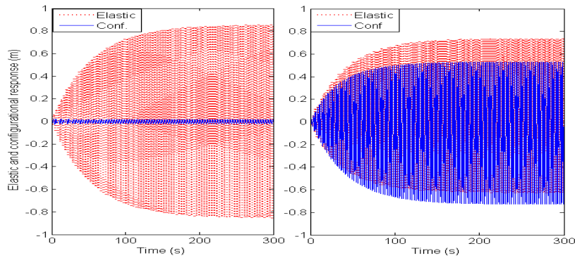
Fig. 7(c): z_4 - waveforms for mode 1 ( \omega_f = 1.84 rad/s) and mode 2 ( \omega_f = 2.56 rad/s).
