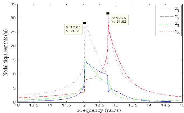
Fig. 5(a): FDR for one-to-one internal resonance with proportional harmonic loading.
