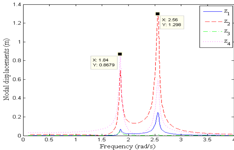
Fig. 7(a): Exact FDR for cables with low sag/span ratio.
