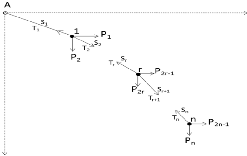
Fig. 1(a): Cable with n nodes fixed at one end.
