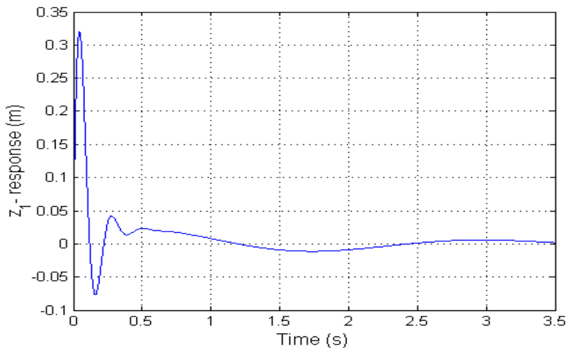
Fig. 2: z_2 - waveform for damped modal vibrations.
