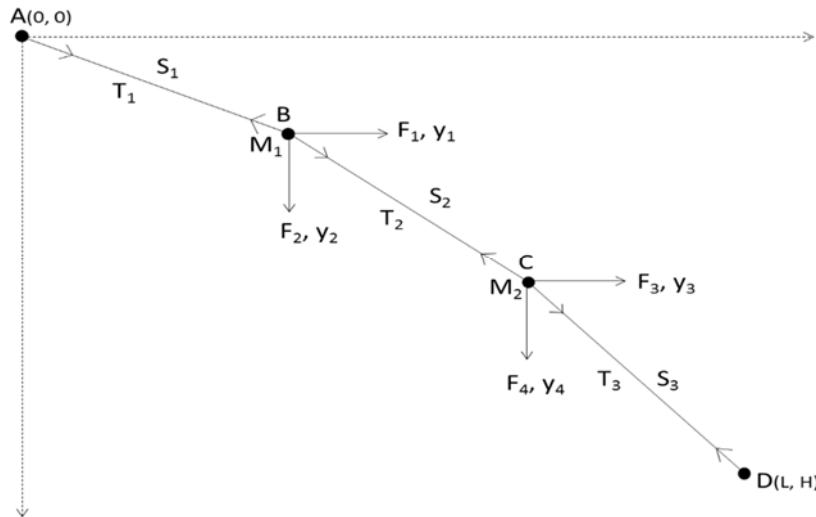
Fig. 1(b): Cable structure fixed at both ends with lumped masses.
