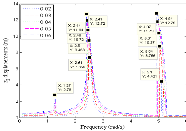
Fig. 4: Effect of peak sinusoidal forces on FDR.
