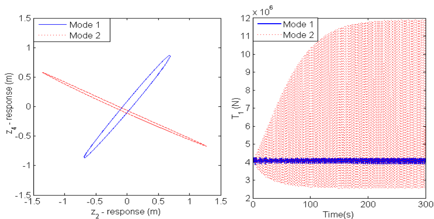
Fig. 7(b): Modal Lissajous plots and modal tension T_1 waveforms.
