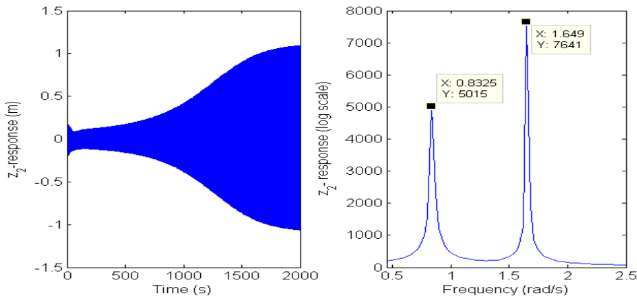
Fig. 8 (c): z_2 - waveform and FFT plot ( \omega=1.62 rad/s).
