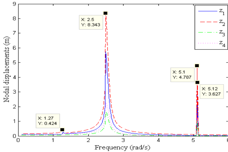
Fig. 3(a): Typical FDR for general forcing function.
