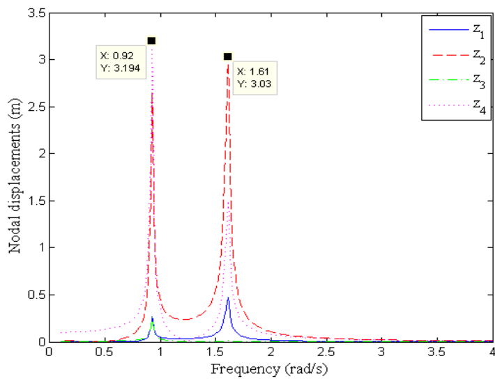
Fig. 6: Approximate FDR for cables with low sag/span ratio.
