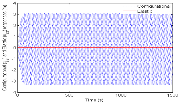
Fig. 8(b): Configurational and elastic response plot ( \omega=0.81 rad/s).
