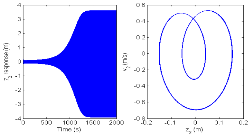
Fig. 3(b): z_2 - waveform and phase plot ( \omega = 5.1 rad/s).
