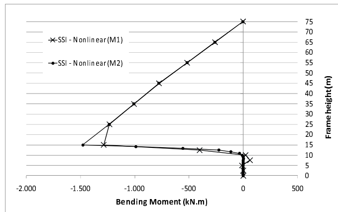
Figure 17 Bending moment along the frames height
