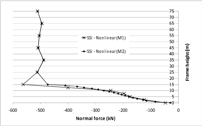
Figure 15 Normal force along the frames height
