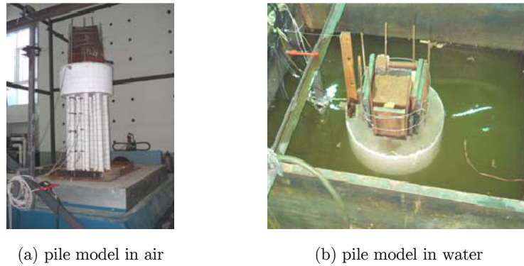
Figure 7: Testing Model.
