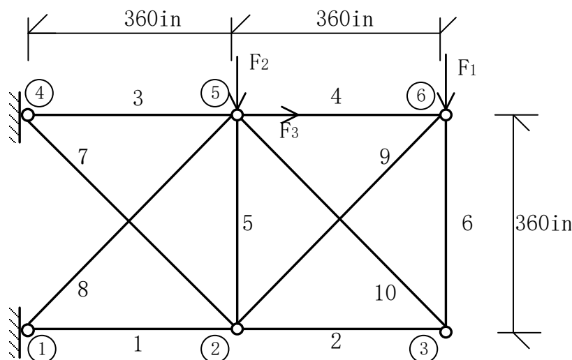
Figure 2: Ten-bar truss with mixed uncertainties
