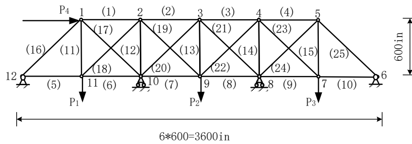
Figure 3: 25 -bar truss with mixed uncertainties
