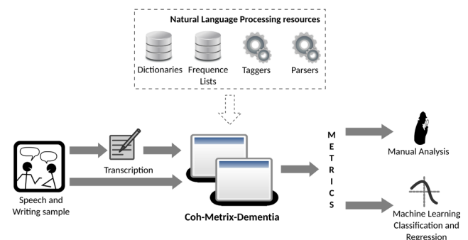
Figure 1. Architecture of Coh-Metrix-Dementia.
