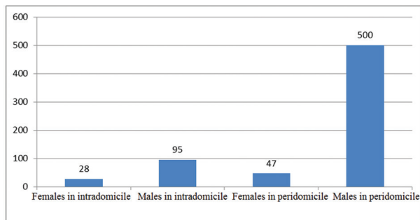
Fig. 2: number of Lutzomyia longipalpis captured in the peri- and intradomicile areas, separated by gender, demonstrating the exophilic and endophilic behaviors of the populations. Northwestern region of Belo Horizonte, Minas Gerais, Brazil.
