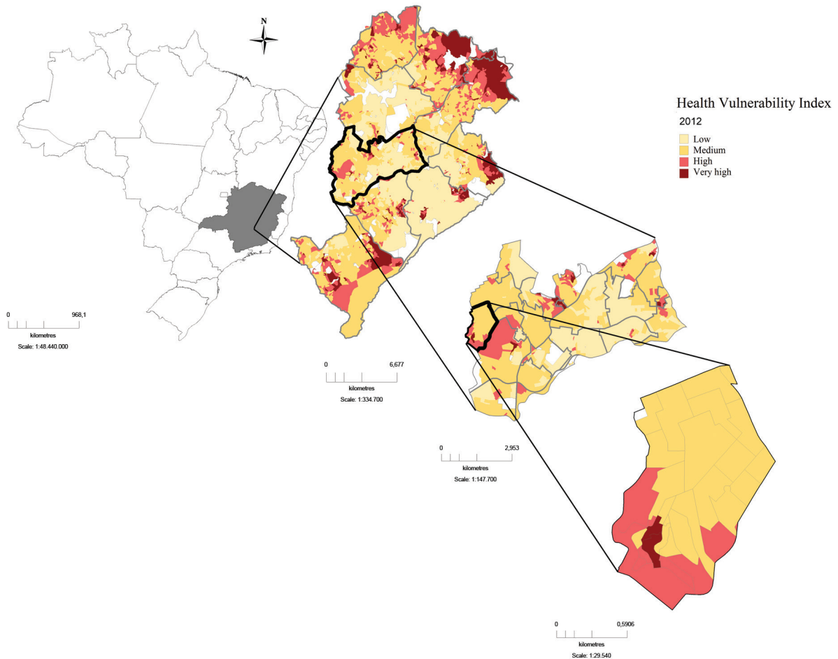
Fig. 1: Vulnerability Index map of Belo Horizonte, Minas Gerais, Brazil, and study area (northwestern region).
