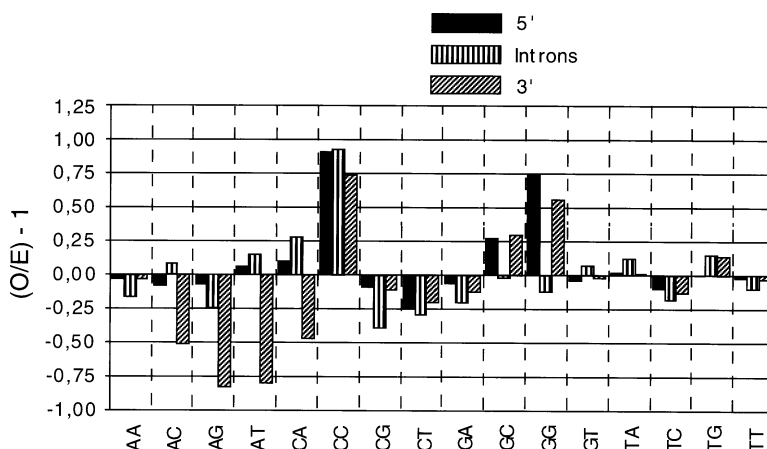
Fig. 5: weight-averaged (Observed/Expected)-1 dinucleotide frequencies for the total sum of 5'- UTR (5'), introns and 3'- UTR (3').
