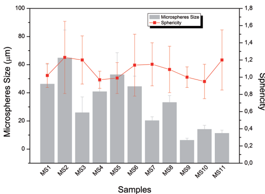
Figure 3: Mean Size and sphericity of the microspheres obtained by different processing conditions tested in the factorial design.
