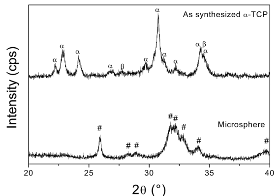
Figure 1: XRD patterns of the as synthesized \alpha -TCP and one microsphere condition obtained by W/O emulsion. ( \alpha : \alpha -TCP, \beta : \beta -TCP, # - CDHA).
