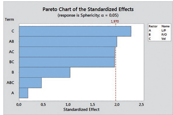
Figure 4: Pareto Chart of the standardized effects with a P-value < 0,05.
