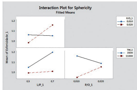
Figure 5: Interaction plot of the factors verified on the factorial design.
