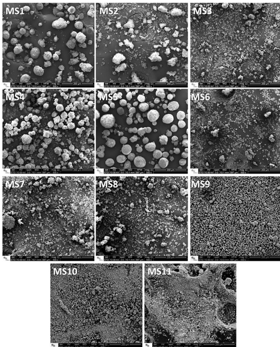
Figure 6: SEM micrographs presenting the microspheres obtained by the different processing conditions tested in the factorial design.
