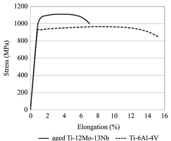
Figure 3. Stress-strain curves of aged Ti-12Mo-13Nb alloy and Ti-6Al4V alloy at room temperature and strain rate of 4 \times 10^{-3} \text{ s}^{-1} .
