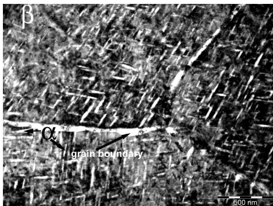
Figure 2. TEM image (bright-field) of Ti-12Mo-13Nb alloy hot swaged and aged at 500 °C/24 h showing a fine distribution of \alpha precipitates in the \beta matrix.
