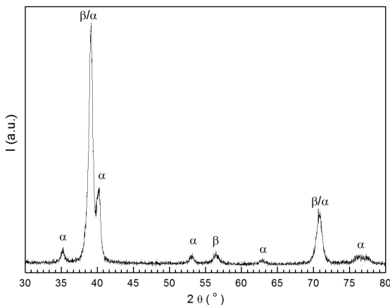
Figure 1. X-ray diffraction pattern of the Ti-12Mo-13Nb alloy hot swaged and aged at 500°C/24 h, showing diffraction peaks from \alpha and \beta phases.
