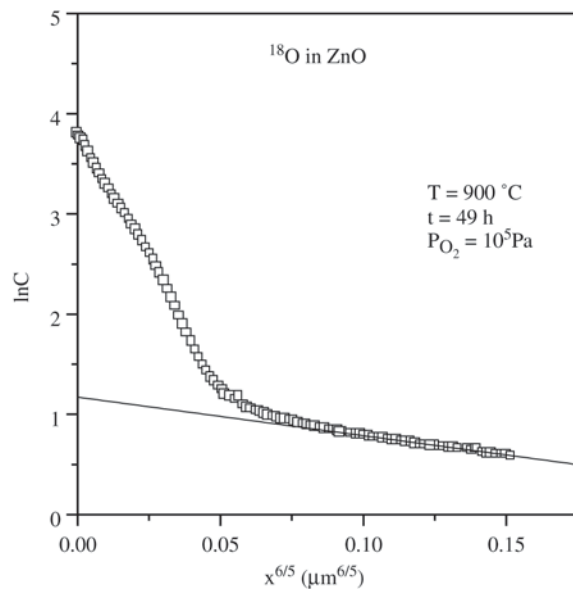
Figure 4. Oxygen concentration plot against x^{6/5} for oxygen diffusion in pure ZnO (900 °C, oxygen pressure 10 5 Pa, 1.764 × 10 5 s).
