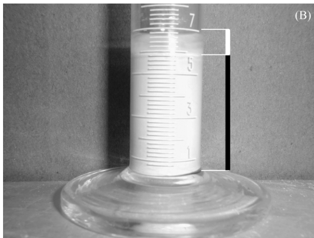
Figure 1. Sedimentation behaviour of two ZrO 2 /stainless steel suspensions: A) 70 wt.% solid loading and 1 wt.% deflocculant, B) 80 wt.% solid loading and 3 wt.% deflocculant.
