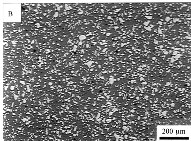
Figure 2. Optical micrographs of the polished cross section of zirconia/stainless steel composites: A) 15 vol.% metal and B) 30 vol.% metal. Lighter phase is metal and the darker phase is zirconia.
