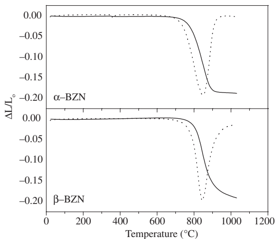
Figure 8. Dilatometric analysis of \alpha -BZN and \beta -BZN powders treated for 2 hours at 700 °C.
