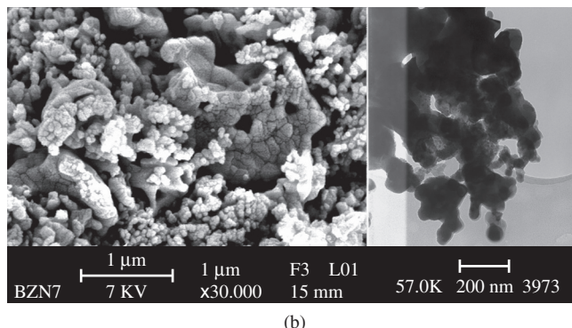
Figure 6. SEM and TEM images of powders treated for 2 hours at 700 °C: a) \alpha -BZN; and b) \beta -BZN.
