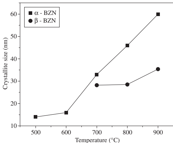
Figure 4. Crystallite size as a function of temperature for \alpha -BZN and \beta -BZN powders.
