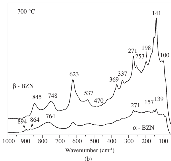
Figure 5. Spectra for \alpha - and \beta -BZN powders heated at 500 and 700 °C, respectively. a) FT-IR; and b) Raman.
