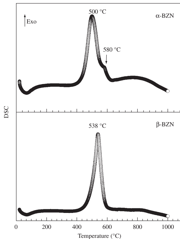
Figure 1. Thermal analysis of BZN powders treated at 400 °C for 4 hours.
