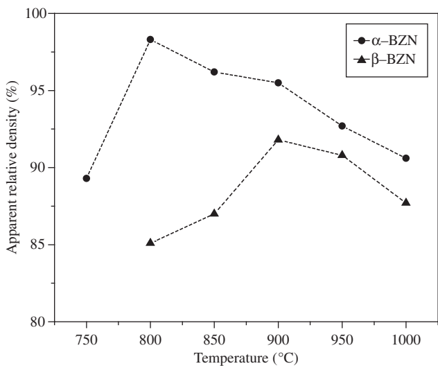
Figure 9. Evolution of apparent relative density of \alpha -BZN and \beta -BZN powders as a function of temperature.
