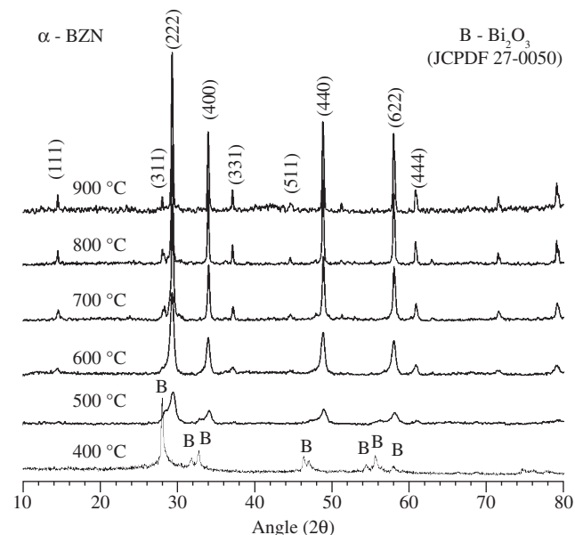
Figure 2. XRD patterns of \alpha -BZN powders treated for 2 hours at temperatures ranging from 400 to 900 °C.
