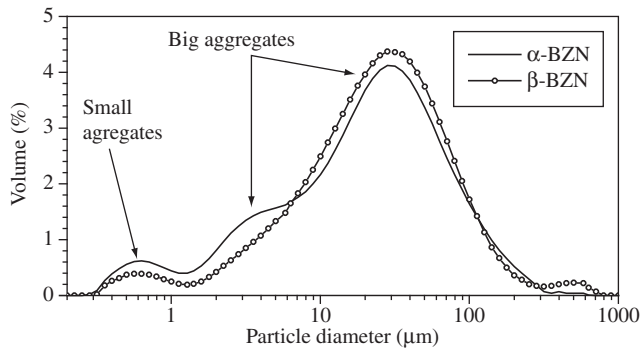
Figure 7. Histogram of particles and aggregates size of BZN samples.
