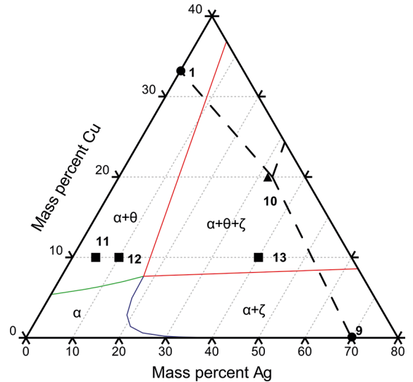
Figure 2. Al-rich corner of Al-Ag-Cu phase diagram. Dashed lines are univariant Al-Ag and Al-Cu binary eutectic reactions. The alloys used in this work are added in the graph.
