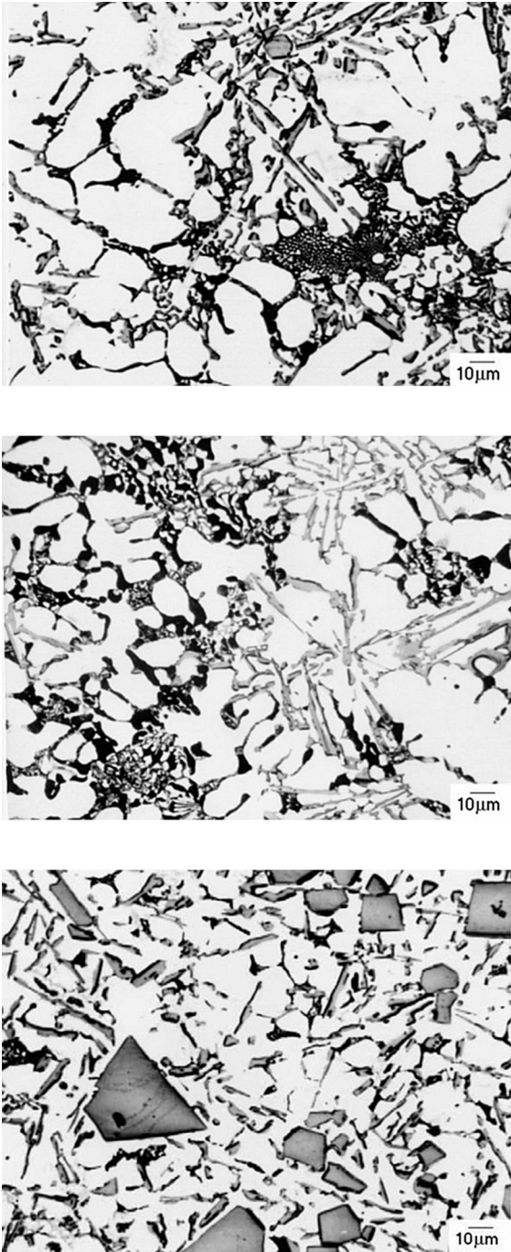
Figure 4. Typical microstructures of longitudinal sections of a) alloy #4 Al-5%Cu-9%Si, b) alloy #5 Al-21%Cu-6%Si; c) alloy #6 Al-5%Cu-12.5%Si; White, grey and black phases are \alpha -Al, Si and \text{Al}_2\text{Cu} respectively; interdendritic fine scale phase is ternary eutectic.
