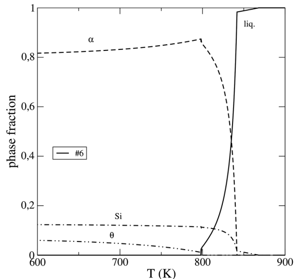
Figure 6. Evolution of molar phase fraction with the temperature during the cooling of the #6 Al-5%Cu-12.5%Si.
