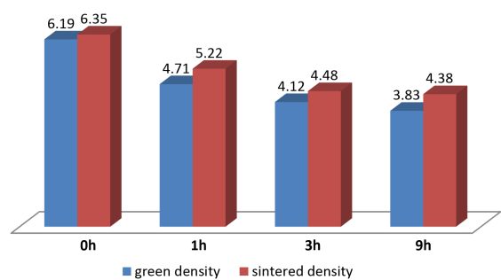
Figure 5. Green and sintered density of specimens.
