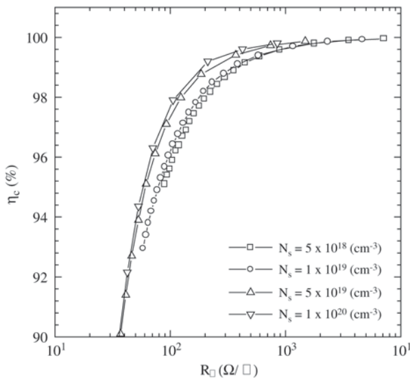
Figure 5. Emitter collection efficiency, \eta_c as function of emitter sheet resistivity, R_{\square} and surface doping level, N_s , considering passivated surfaces.
