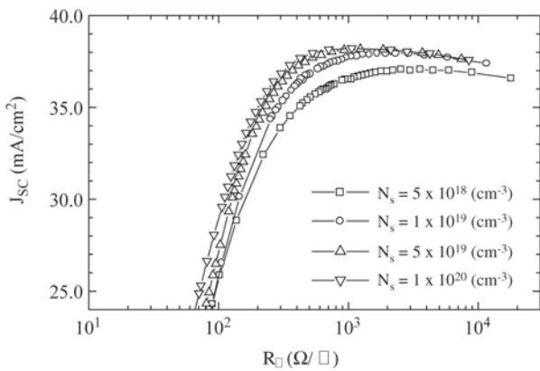
Figure 6. Short-circuit current density, J_{sc} as function of emitter sheet resistivity, R_{\square} and surface doping level, N_s , considering p-type emitter solar cells.
