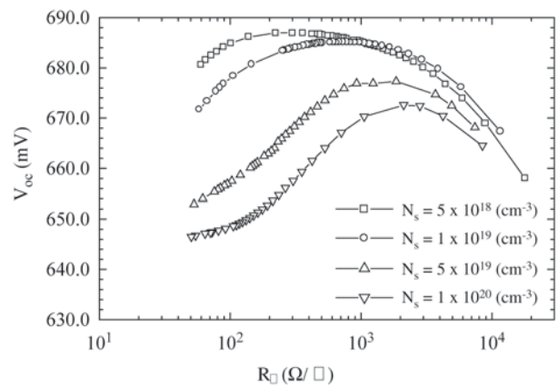
Figure 7. Open circuit voltage, V_{oc} as function of emitter sheet resistivity, R_{\square} and surface doping level, N_s , considering p-type emitter solar cells.
