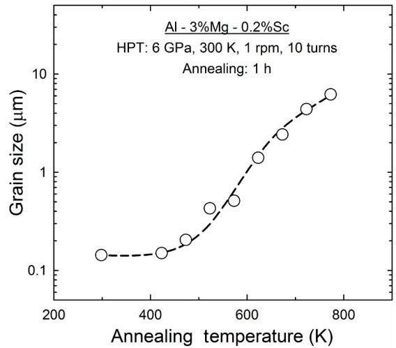
Figure 3. Grain size as a function of annealing temperature for the Al-3Mg-0.2Sc alloy subjected to 10 turns of HPT processing at 300 K and further annealed for 1 h at temperatures from 423 to 773 K.
