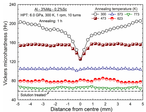
Figure 1. Variation of the average microhardness recorded at the middle-section position with distance from the centre of the Al-3Mg-0.2Sc discs after HPT processing at 300 K and further annealing.
