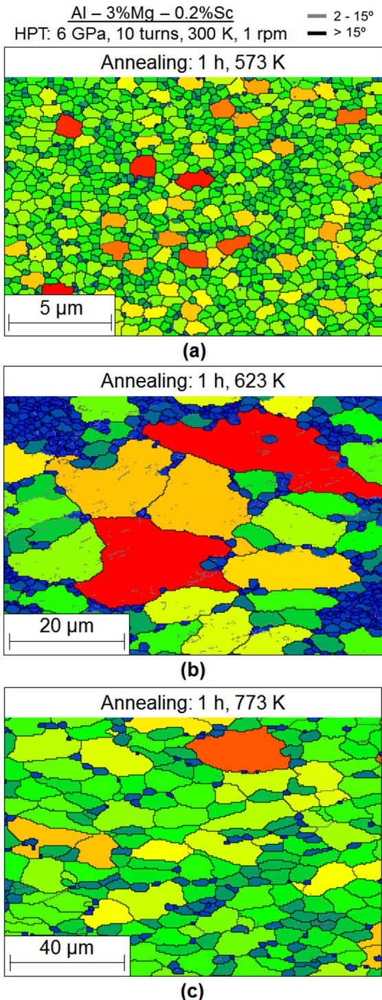
Figure 4. Grain size coloured images of the grain structures of the Al-3Mg-0.2Sc alloy processed by HPT at 300 K and further annealed for 1 h at (a) 573, (b) 623 and (c) 773 K.
