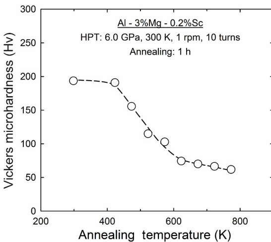
Figure 2. Average microhardness as a function of annealing temperature for the Al-3Mg-0.2Sc alloy subjected to 10 turns of HPT processing at 300 K and further annealed for 1 h at temperatures from 423 to 773 K.
