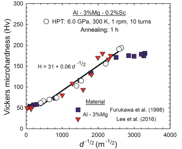
Figure 5. Plot of Vickers microhardness as a function of d^{-1/2} for the Al-3Mg 12,35 and the Al-3Mg-0.2Sc alloy after HPT processing at ambient temperature and after HPT followed by annealing for 1 h at temperatures ranging from 423 to 773 K.
