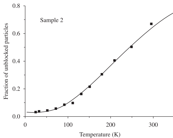
Figure 3. Temperature dependence of the volume fraction of unblocked particles in sample 2 of Table 1 (annealed at 400 °C), calculated from the Mössbauer spectra. The dots are experimental points; the line is a fit to a cumulative log-normal function (see text).
