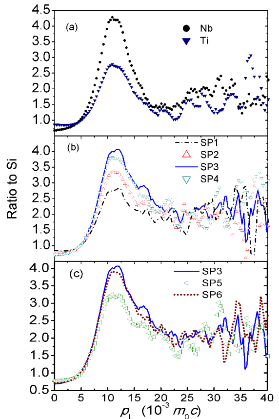
Figure 4. The ratio curves for the samples; (a) Nb and Ti ratio curves; (b) The SP1, SP2, SP3 and SP4 ratio curves, (c) The SP3, SP5 and SP6 ratio curves; The reference sample is Si.
