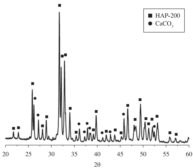
Figure 2. X-ray diffraction patterns of POVIAC ® /CaCO 3 /HAP-200 composite.
