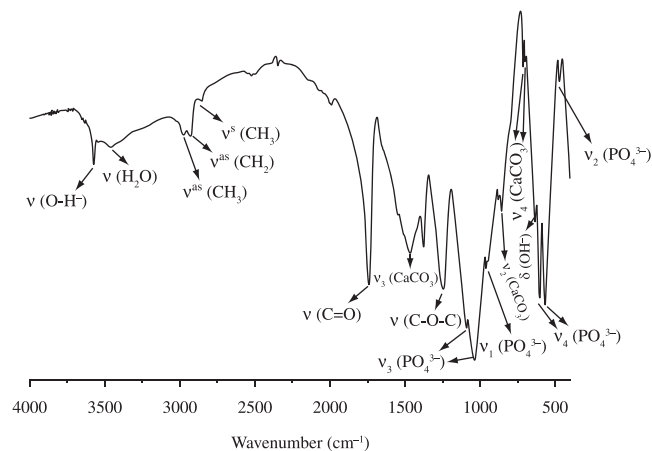
Figure 1. FT-IR spectra of the POVIAC®/CaCO 3 /HAP-200 composite.
