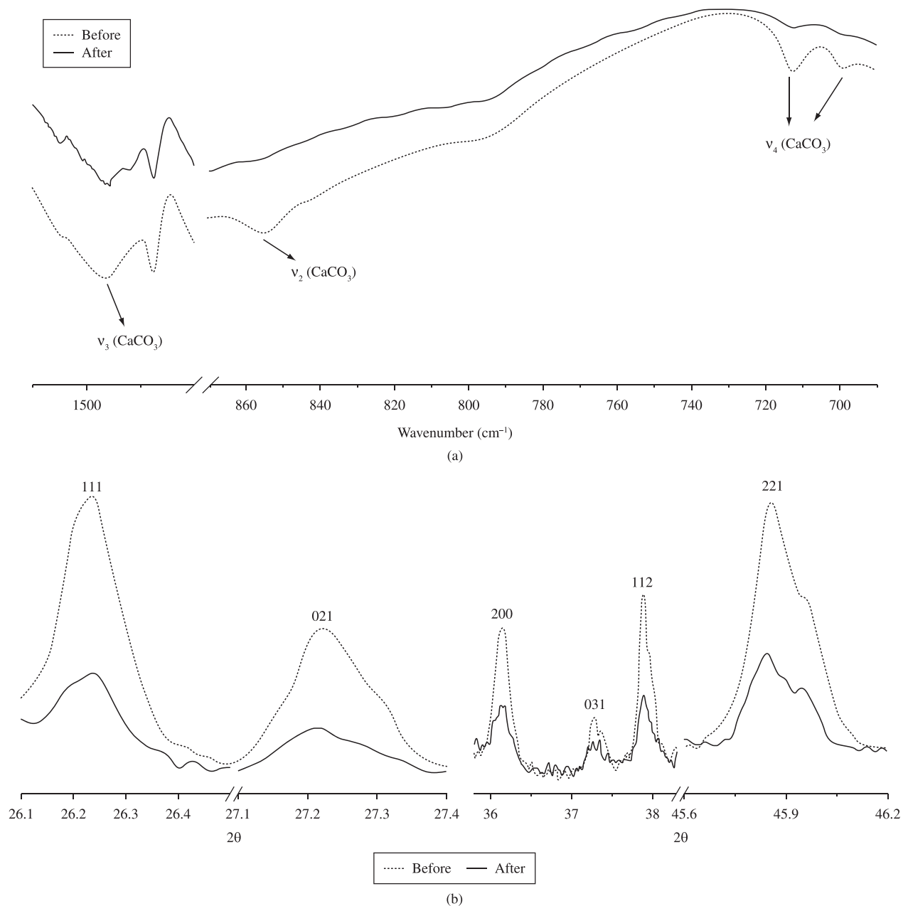
Figure 6. Physicochemical characterizations of POVIAC ® /CaCO 3 /HAP-200 composite, before and after soaking in SBF for 30 days: a) FT-IR analyses; and b) X-ray diffraction patterns.
