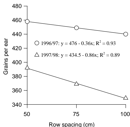
Figure 1. Row spacing effect on the number of grains per ear of maize in Southern Brazil, during the growing seasons of 1996/97 and 1997/98. Lages, SC.
