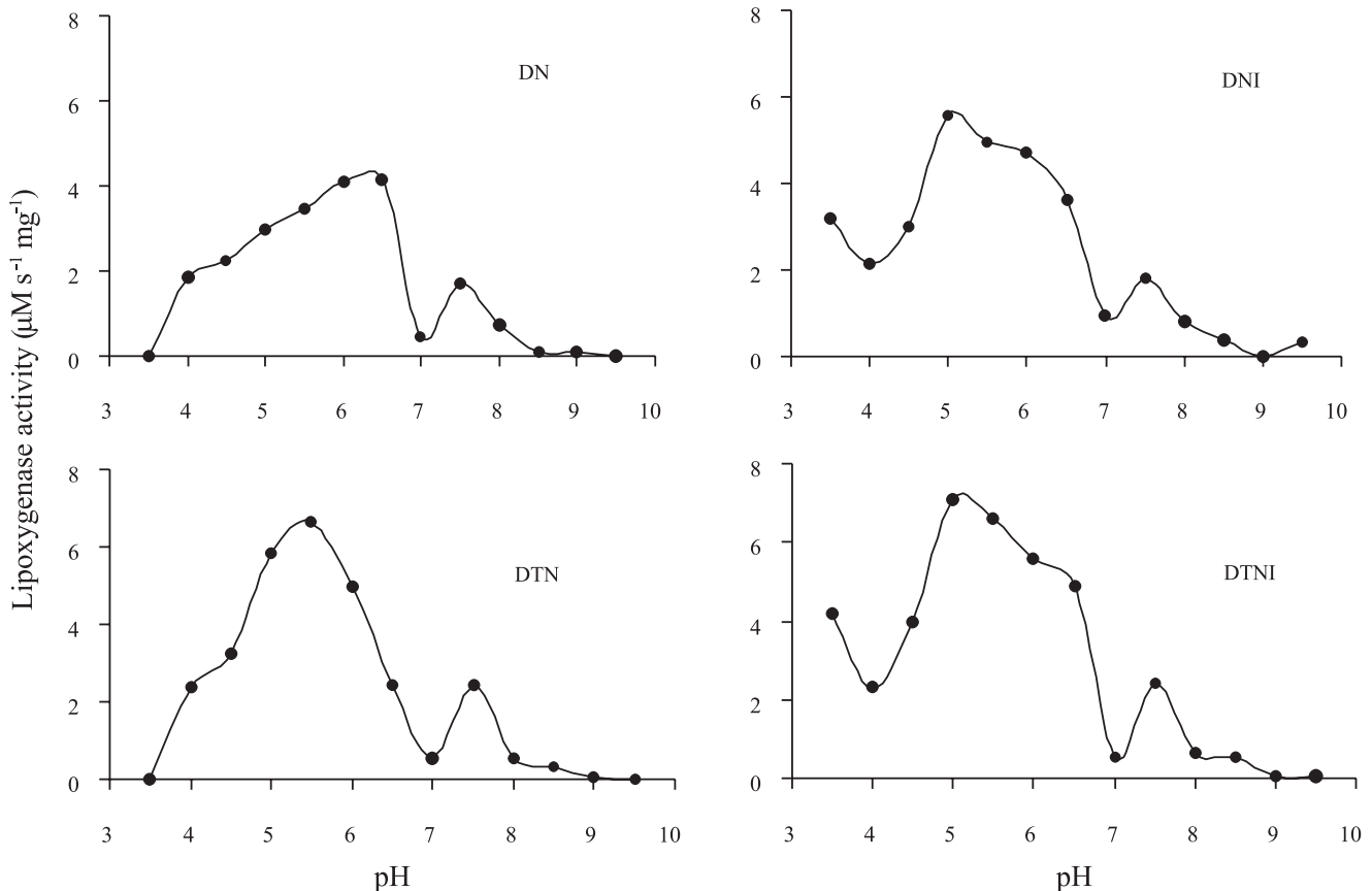
Figure 1. Specific lipoxygenase activity in roots from the Doko (DN), Doko inoculated (DNI), Doko triple-null (DTN) and Doko triple-null inoculated (DTNI) soybean lines 28 days post-inoculation at different pH values.
