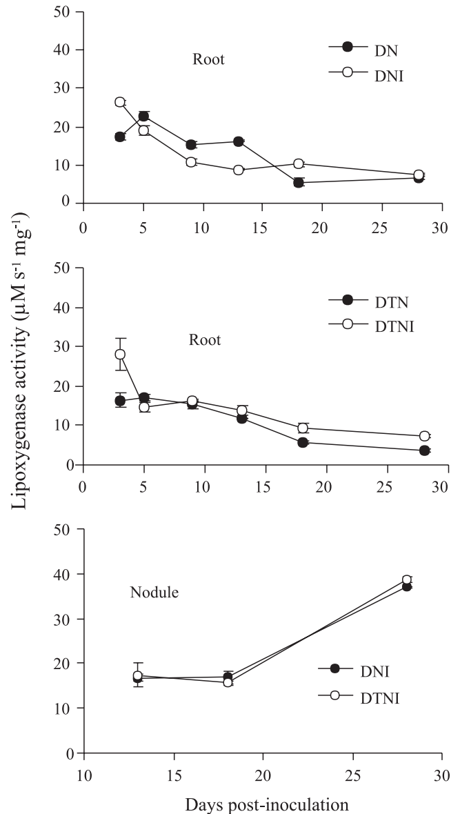
Figure 3. Lipoxygenase activity in roots and nodules from Doko (DN), Doko inoculated (DNI), Doko triple-null (DTN) and Doko triple-null inoculated (DTNI) soybean lines at different developmental stages.
