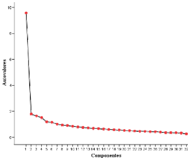
Figura 1. Scree Plot
