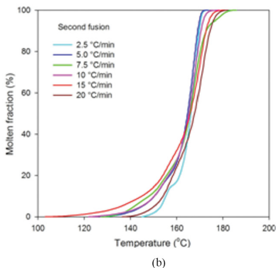
Figure 8. Evolution of molten fraction with time (a) and temperature (b) for the melting event during the reheating stage ( F_2 ).
