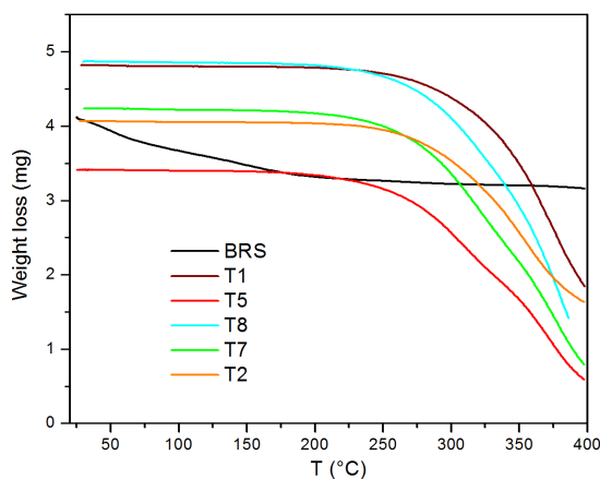
Figure 2. TGA analysis for the resol phenolic resins synthesized from extracts.
