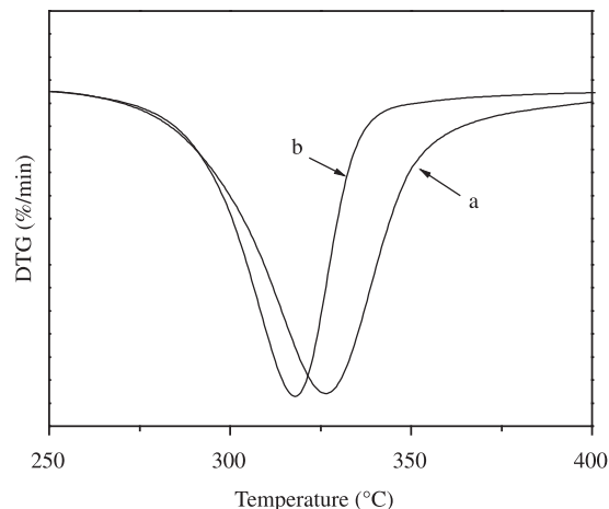
Figure 6. DTG curves of PBLG/PAA blend films with two PAA mole contents: (a) 0 and (b) 14%.
