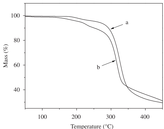
Figure 5. TG curves of PBLG/PAA blend films with two PAA mole contents: (a) 0 and (b) 14%.
