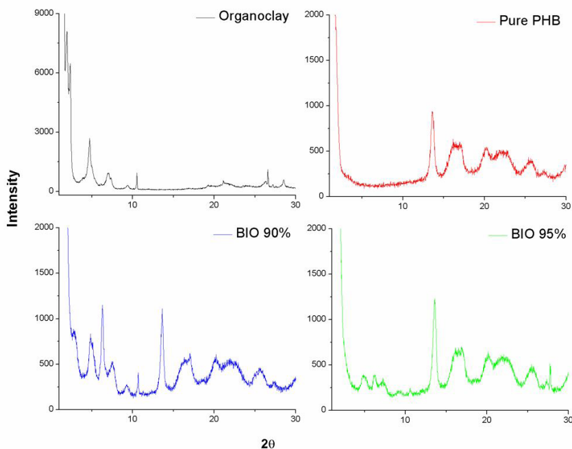
Figure 2. Diffractograms of the organoclay and the pure PHB and bionanocomposites films.
