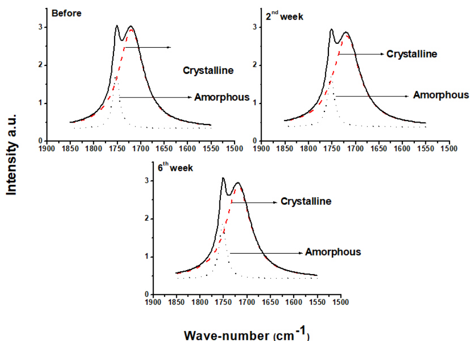
Figure 4. BIO 95% spectra after deconvolution (C=O carbonyl band) before and after degradation.
