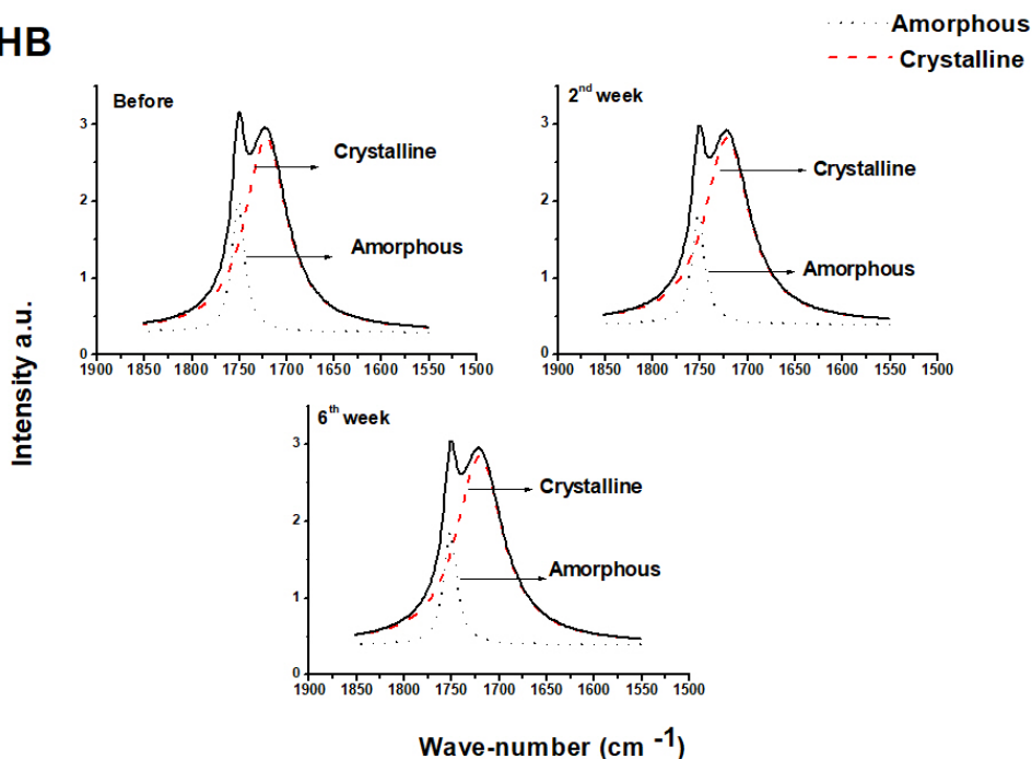
Figure 3. PHB spectra after deconvolution (C=O carbonyl band) before and after degradation.
