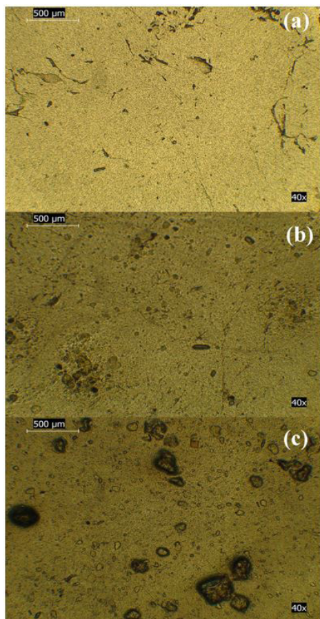
Figure 1. Optical micrographs of the (a) pure PHB, (b) BIO 95% and (c) BIO 90% films.
