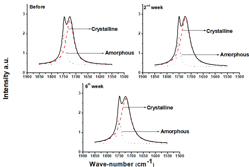
Figure 5. BIO 90% spectra after deconvolution (C=O carbonyl band) before and after degradation.
