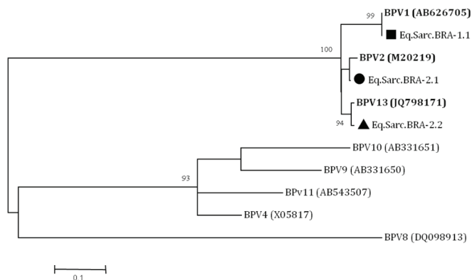
Fig.1. Phylogenetic tree obtained by the maximum-likelihood method based on the nucleotide sequences of a 197 bp fragment within PVs E5L2 gene. Bootstrap values are indicated when at least 50% as a percentage was obtained from 1,000 replications. The BPVs strains are marked according to the BPV cluster: BPV1 (square), BPV2 (circle), and BPV13 (triangle). The other samples, not included on figure, presented similar sequences. The E5L2 sequences were not submitted in GenBank because the fragment is shorter than 200bp in length. BPV sequence names are labelled as follows: BLAST identification and GenBank accession number. The scale bar represents a genetic distance of 0.1 substitutions per site.
