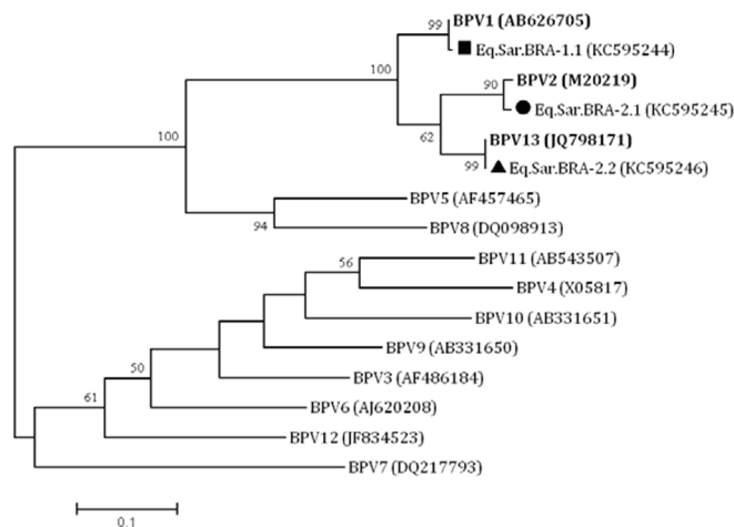
Fig.2. Phylogenetic tree obtained by the maximum-likelihood method based on the nucleotide sequences of a 341 bp fragment within BPV L1 gene, 5558 to 6013 nt of BPV1, 5725 to 6199 nt of BPV2 and 5745 to 6219 nt of BPV13. Bootstrap values are indicated when at least 50% as a percentage was obtained from 1,000 replications. The BPV strains from Deltapapillomavirus genus identified in equine sarcoids Eq.Sarc.BRA-1.1, Eq.Sarc.BRA-2.1, and Eq.Sarc.BRA-2.2 are marked as square, circle, and triangle, respectively. The other samples, which were not included on figure, presented similar sequences. BPV sequence names are labelled as follows: BLAST identification and GenBank accession number. The scale bar represents a genetic distance of 0.1 substitutions per site.
