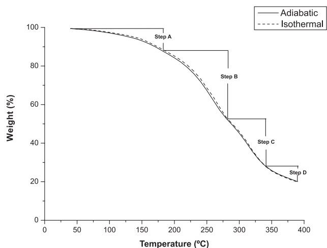
Figure 5. Thermogram of the effect of temperature on weight loss of the 0.40 G/WG bioplastics
