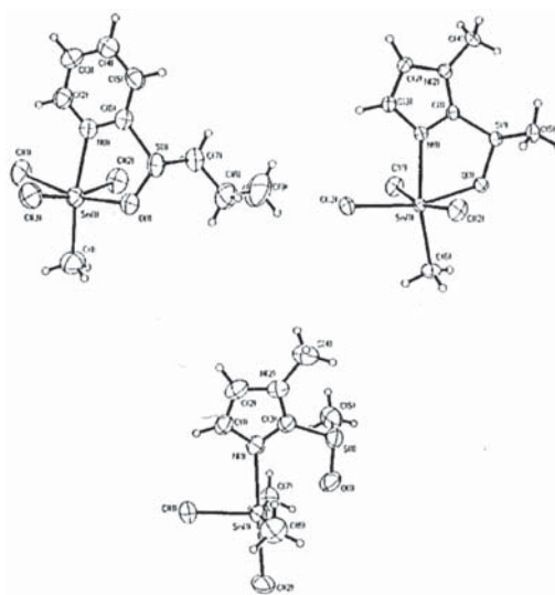
Figura 7. Estruturas dos complexos \text{MeSnCl}_3 \cdot \text{ImSOMe} , \text{MeSnCl}_3 \cdot \text{PySOPr} e \text{Me}_2\text{SnCl}_2 \cdot \text{ImSOMe} .
