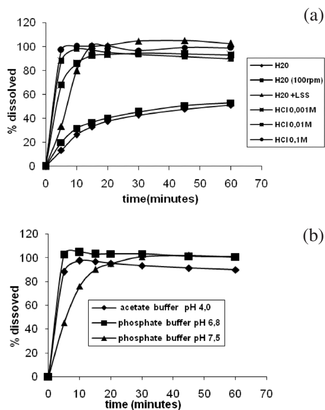
Figure 3. Dissolution profiles of telithromycin tablets using H 2 O, H 2 O + SLS, 0,001M HCl, 0,01M HCl, 0,1M HCl (a), acetate buffer pH 4.0, phosphate buffer pH 6.8 and 7.5 (b) in apparatus 2, rotating 50 rpm
