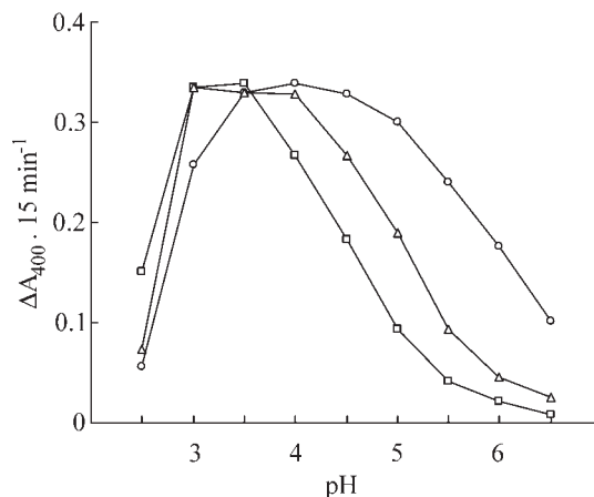
Figure 2. Enzyme activity as a function of the assay medium pH of partially purified cotyledonary \beta -galactosidases extracted from Pitiúba cowpea, Vigna unguiculata (L.) Walp., quiescent seeds. \beta -gal I (o), \beta -gal II ( \square ) and \beta -gal III ( \Delta ). Values represent the mean of three different experiments with three replicates each.
