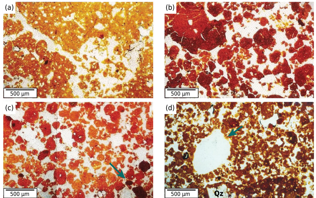
Figure 5. Photomicrographs of the Ap horizon (a), BA horizon (b), Bw 2 horizon (c), and Bw 3 horizon (d) in the P 3 - Geric Acric Rhodic Ferralsol (Clayic, Dystric); Serra do Salitre topolithosequence. Ap horizon showing a strongly coalesced granular structure (a), BA horizon showing a typical oxic microstructure (b), with larger aggregates compared with the underlying Bw 2 (the arrow shows a Ti/Fe nodule) (c), and for the Bw 3 horizon, aggregates are significantly smaller with abundant oriented, striated clay plasma, as dispersed clay and biological channels (arrow) (d). Qz: quartz.
