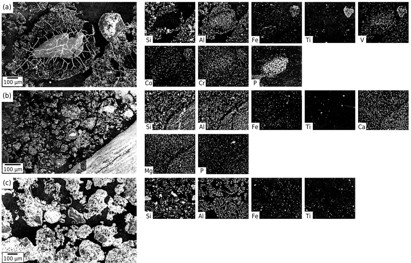
Figure 4. Scanning electron microscope photomicrographs and EDS microchemical maps of the Bi horizon in the P 2 - Eutric Chromic Leptic Cambisol (Humic, Loamic); Serra do Salitre topolithosequence. Degraded apatite grains within microaggregates (a), micro-quartz veins in lithorelict fragments (b), and quartz grains within a well-developed granular structure (c).
