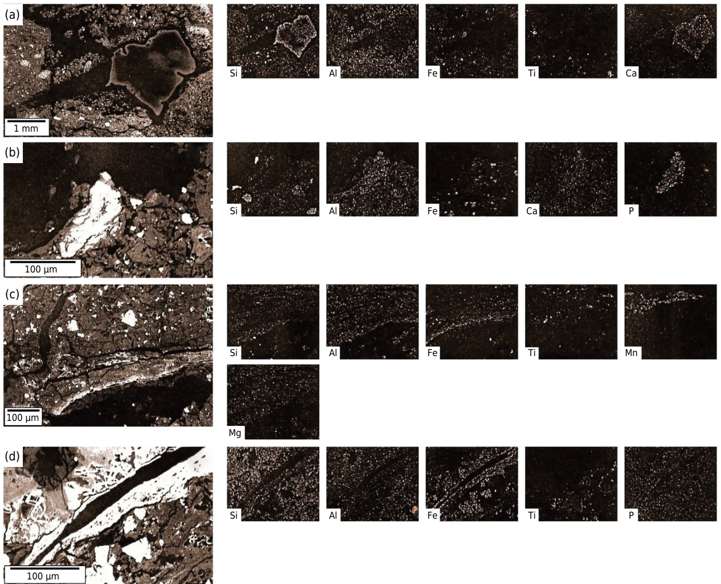
Figure 10. Scanning electron microscope photomicrographs and EDS microchemical maps of the Bi horizon in the P_6 - Eutric Chromic Petrolintic Leptic Cambisol (Clayic, Humic); Coromandel topolithosequence. Volcanic glass rich in Si and Ca (a), apatite grains partially weathered (b), and illuvial coatings (ferrans and mangans) (c and d).
