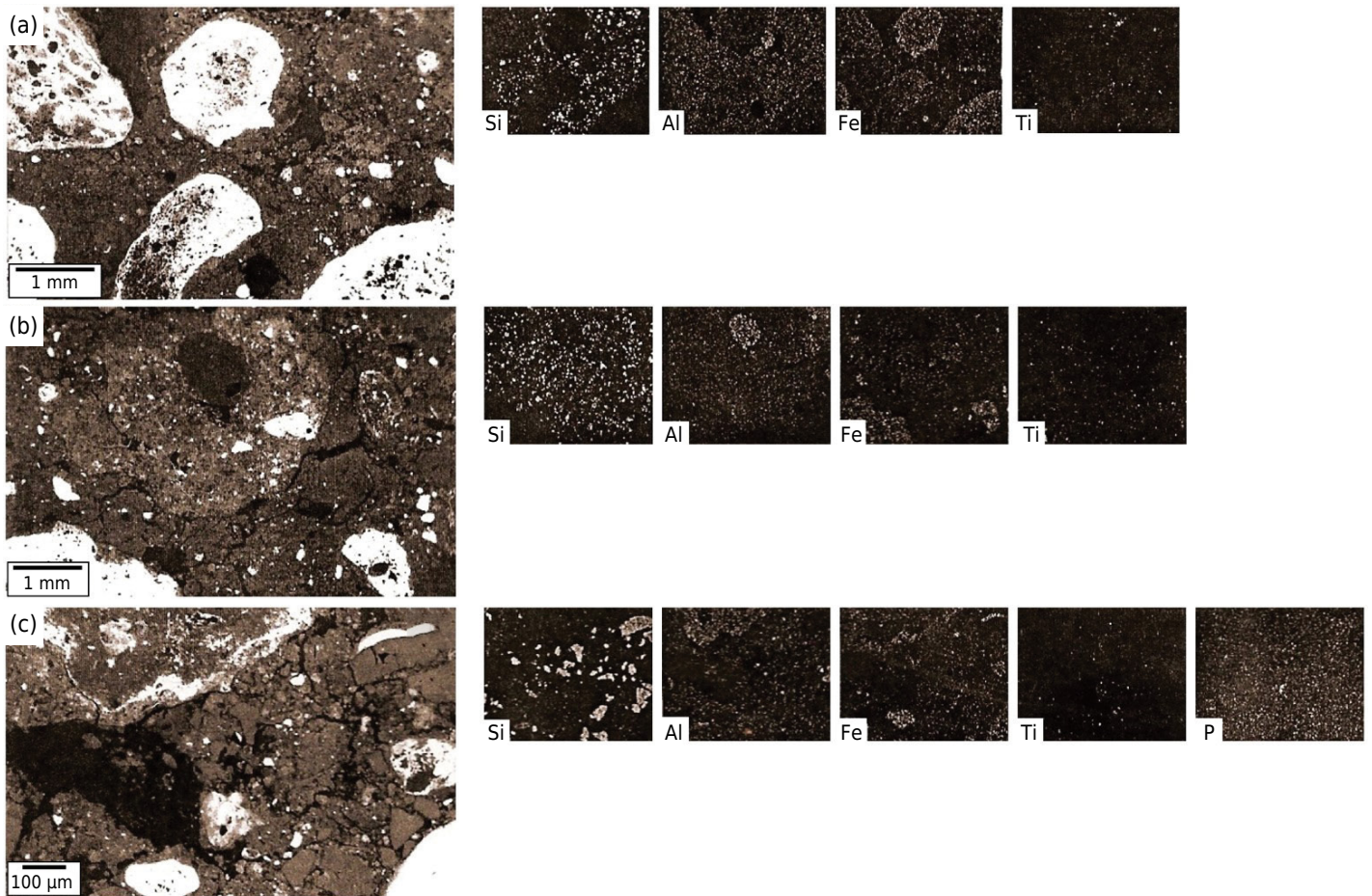
Figure 12. SEM photomicrographs and EDS microchemical maps of the Bw 2 horizon in the P 7 - Geric Rhodic Petroplinthic Ferralsol (Clayic, Dystric); Coromandel topolithosequence. Sand-sized micronodules (a and b), and quartz and P-rich grains (c).
