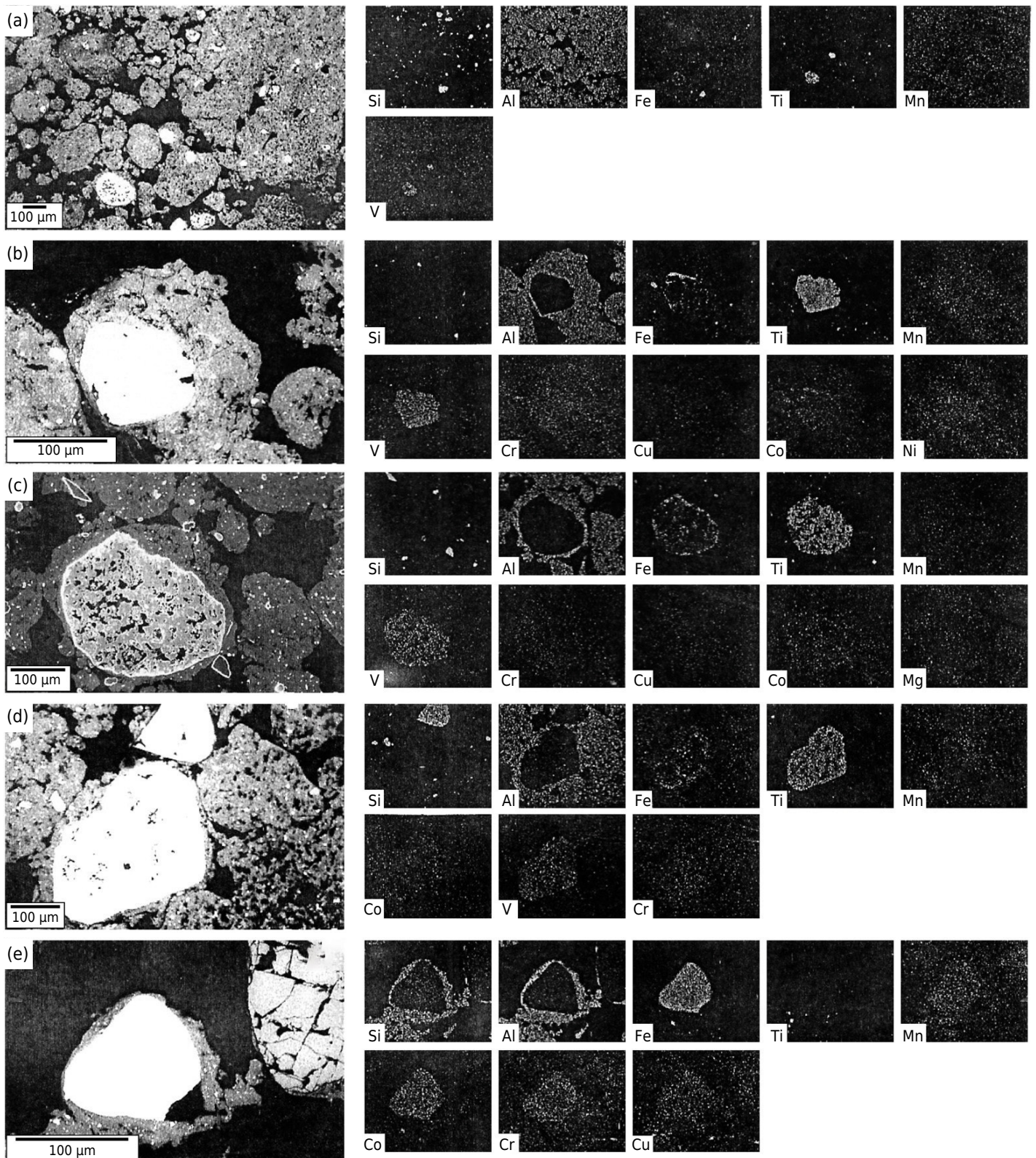
Figure 6. Scanning electron microscope photomicrographs and EDS microchemical maps of the Bw_2 horizon in the P_3 - Geric Acric Rhodic Ferralsol (Clayic, Dystric); Serra do Salitre topolithosequence. Well-developed oxic microstructure (a), a higher content of iron at the edges of the leucoxene grains (b, c, and d), and ferruginous concretions (e).
