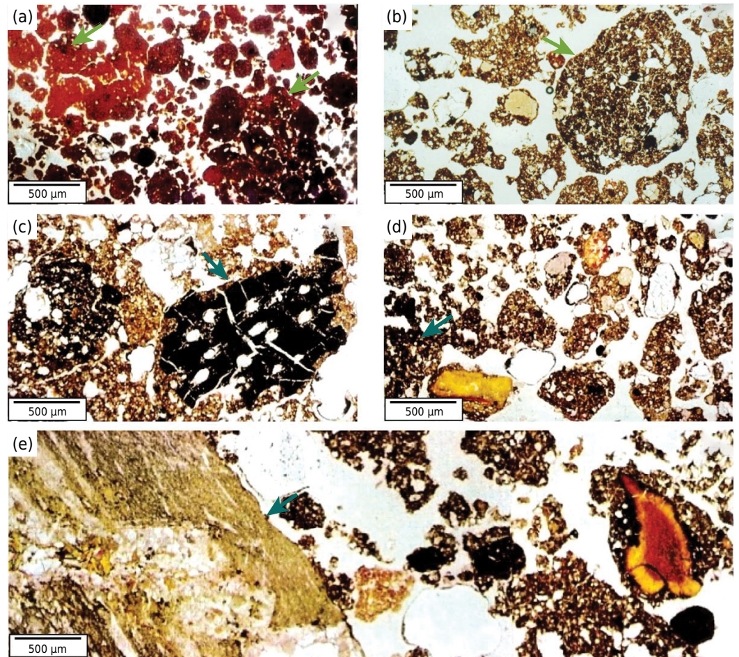
Figure 2. Photomicrographs of the Bw_2 horizon (a) in the P_1 - Acric Rhodic Ferritic Ferralsol (Clayic, Dystric) and of the Bi horizon (b, c, d, and e) in the P_2 - Eutric Chromic Leptic Cambisol (Humic, Loamic); Serra do Salitre topolithosequence. Arrows indicate pelletized materials filling and charcoal microfragments (a), well-developed microgranular structure in the cambic horizon (b), charcoal fragment (c), humified organic remains (d), and fragments from acid metapelitic rocks mixed with altered and pedoplasmated material of volcanic origin (e).
