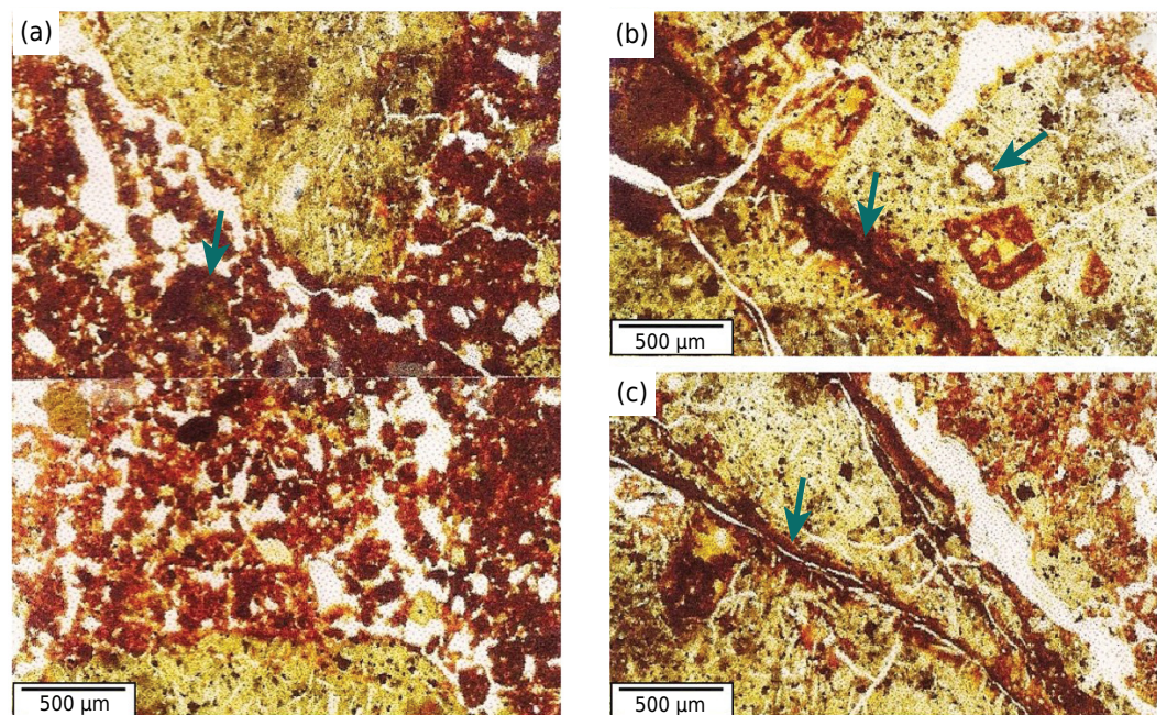
Figure 9. Photomicrographs of the Bi horizon in the P 6 - Eutric Chromic Petroplintic Leptic Cambisol (Clayic, Humic); Coromandel topolithosequence. Arrows indicate well-developed granular structure (a), and mangans and ferrans commonly found along pores, and coating grains (b and c).
