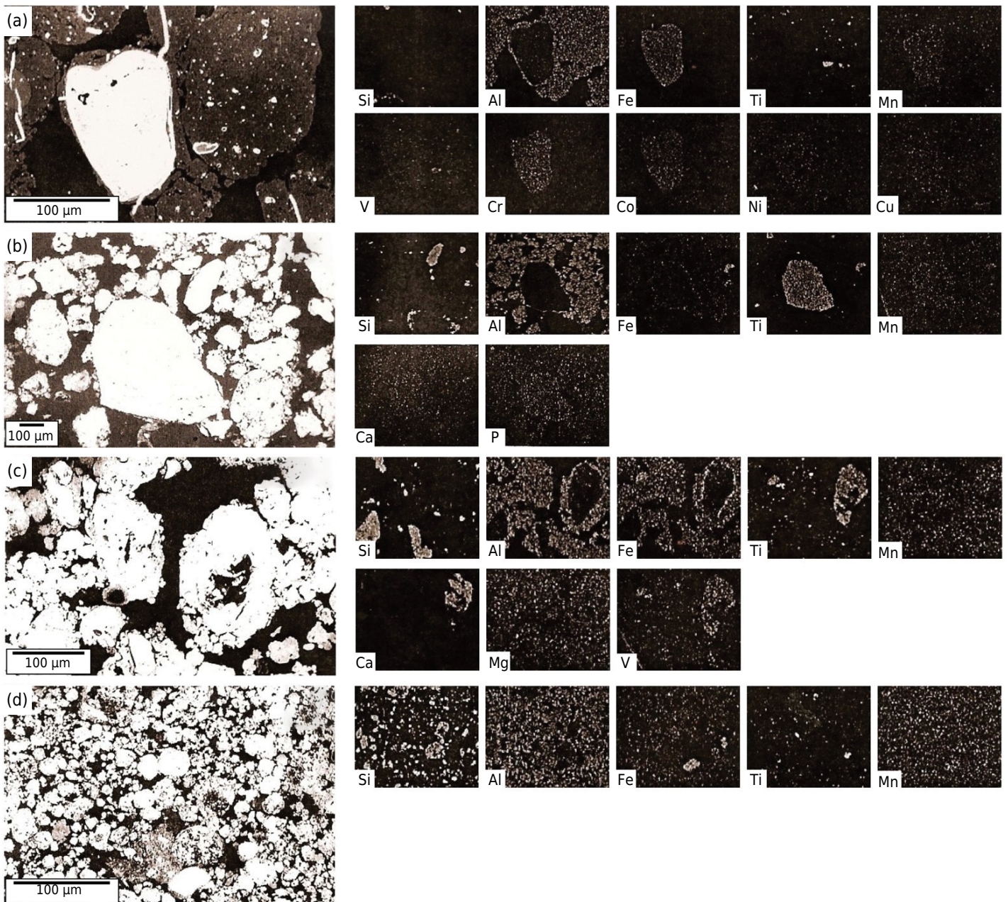
Figure 8. Scanning electron microscope photomicrographs and EDS microchemical maps of the Bw_2 horizon (a and b) in the P_4 - Geric Acric Gibbsic Ferralsol (Clayic, Dystric), and of the Bw_2 horizon (c and d) in the P_5 - Acric Rhodic Ferritic Ferralsol (Clayic, Dystric, Humic); Patrocínio topolithosequence. Fe/Cr-rich alteromorphs (a) and Ti minerals occurring as inclusions in the microaggregates (b), Ti-rich alteromorphs/perovskite (c), and Ti/Fe grains (d).
