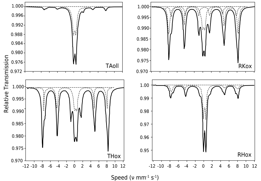
Figure 5. ^{57}\text{Fe} Mössbauer spectra at \sim 298 K for samples from the diagnostic soil horizons.
