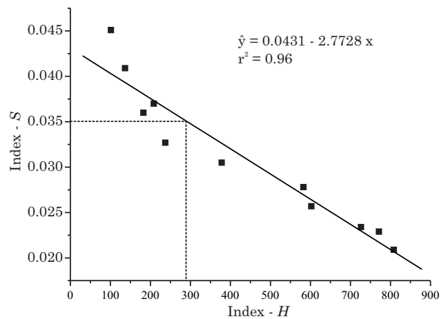
Figure 6. Illustration of negative linear dependence between the indexes S and H . The dashed line shows the S value of 0.035 and the corresponding H value.
