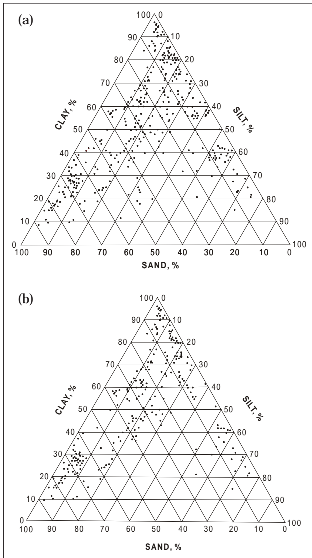
Figure 1. Plots of the soils by their texture (particle size distribution): (a) all samples, (b) samples of A and B horizons of Ferralsols.
