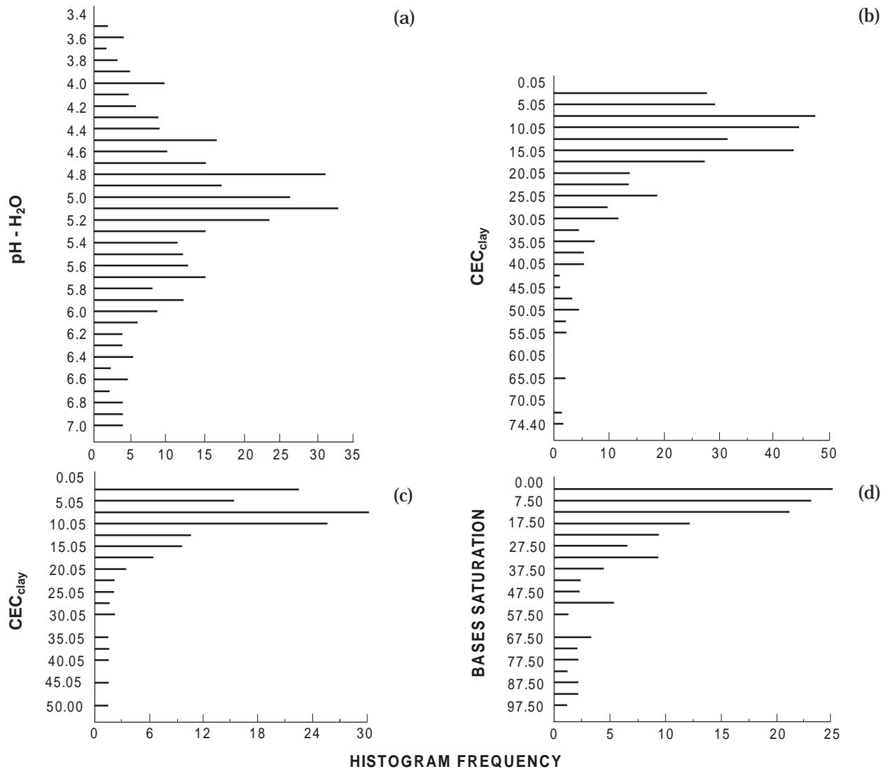
Figure 3. Frequency distribution histogram of pH (a) and CEC_{clay} (b) for all samples analysed and CEC_{clay} (c) and base saturation (d) of soils with Ferralic B horizons.
