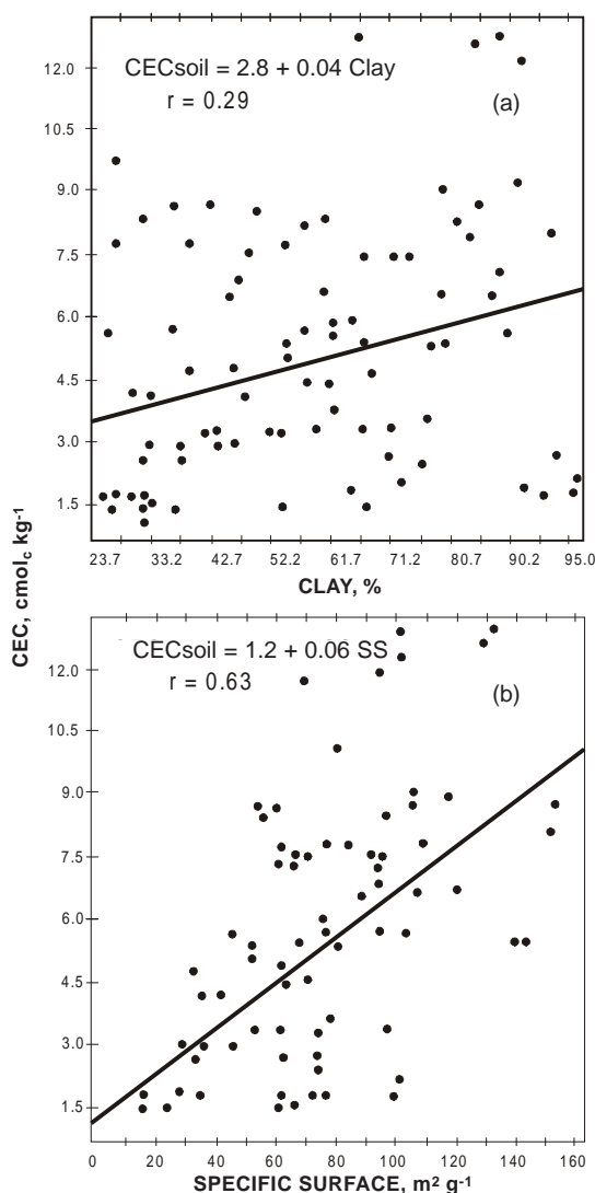
Figure 5. Correlation between: (a) CEC of Ferrallic B horizons and clay content, (b) CEC of Ferrallic B horizons and specific surface area.
