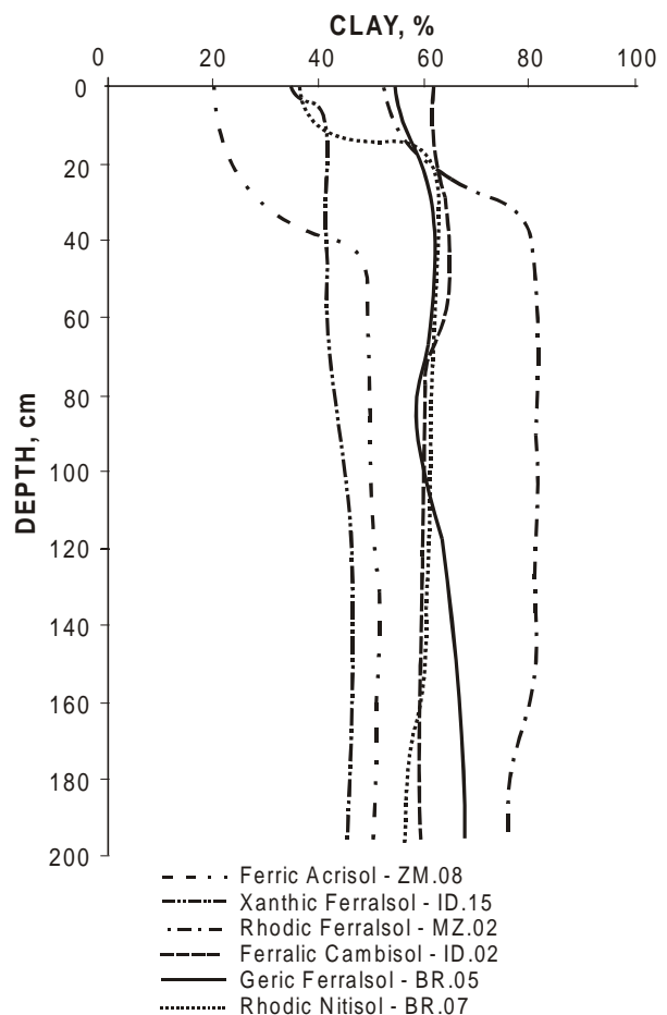
Figure 2. Clay distribution in profiles of representative upland soil of humid and subhumid tropical regions.
