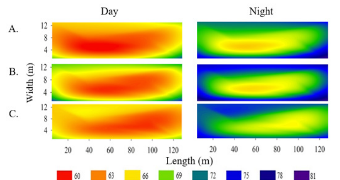
Figure 4. Maps of air relative humidity (%) distribution across the poultry house in the day- and nighttime periods. Mean air humidity in the first week (A), mean air humidity in the second week (B) and mean air humidity in the third week (C)
