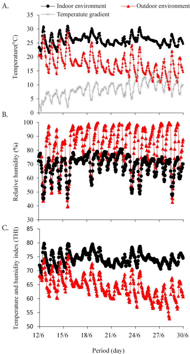
Figure 3. Mean air temperature and the difference between the mean indoor and outdoor air temperature (mean \Delta T ) (A), mean air relative humidity (B), and mean temperature-humidity index (C) in the indoor and outdoor environments of the poultry house
