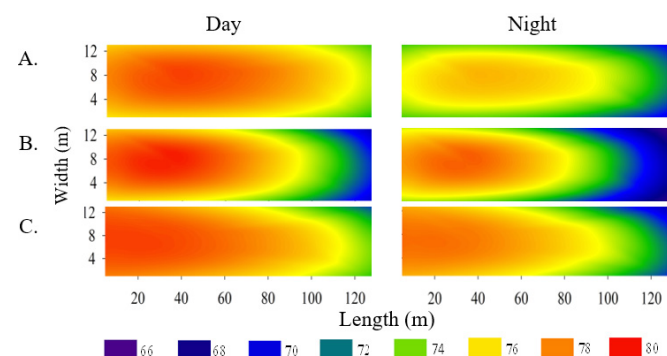
Figure 5. Maps of temperature-humidity index (THI) distribution across the poultry house in the day- and nighttime periods. Mean THI in the first week (A), mean THI in the second week (B) and mean THI in the third week (C)
