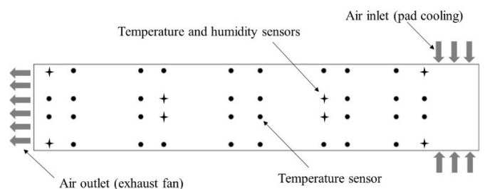
Figure 1. Layout of the ventilation system and arrangement of air temperature/relative humidity sensors inside the poultry house
