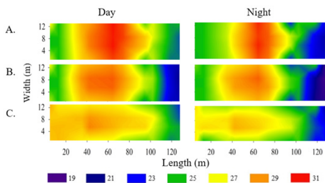
Figure 2. Maps of air temperature ( ^{\circ}\text{C} ) distribution across the poultry house in the day- and nighttime periods. Mean temperature in the first week (A), mean temperature in the second week (B) and mean temperature in the third week (C)
