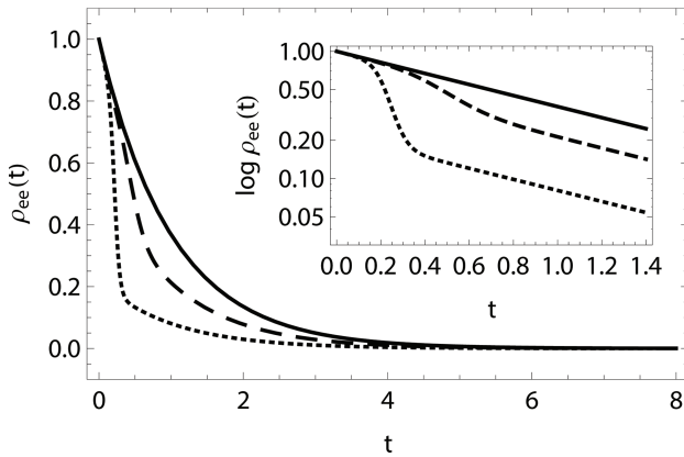
Figure 2 - Excited state probability as function of time including dissipation. We set \Gamma = 1 and \bar{n} = 0 . Solid line: N = 1 ; dashed line: N = 20 ; dotted line: N = 40 .
