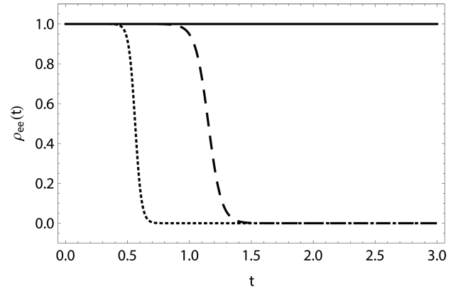
Figure 1 - Excited state probability as function of time in the absence of dissipation. We set \Gamma = 1 . Solid line: N = 1 ; dashed line: N = 20 ; dotted line: N = 40 .
