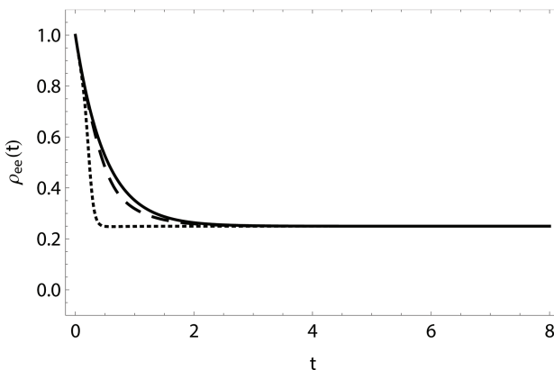
Figure 3 - Excited state probability as function of time including dissipation. We set \Gamma = 1 and \bar{n} = 0.5 . Solid line: N = 1 ; Dashed line: N = 20 ; Dotted line: N = 40 .
