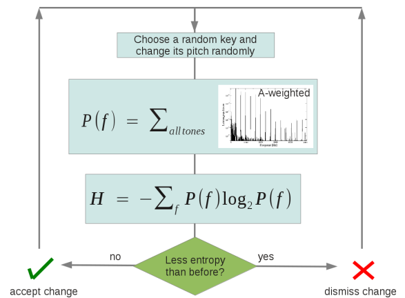
Figure 8 - Monte-Carlo scheme.
