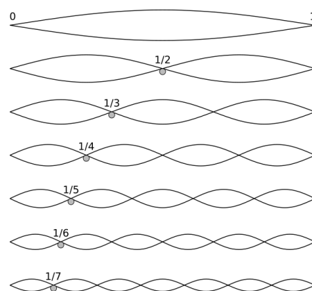
Figure 2 - Harmonic modes of a string [4].
