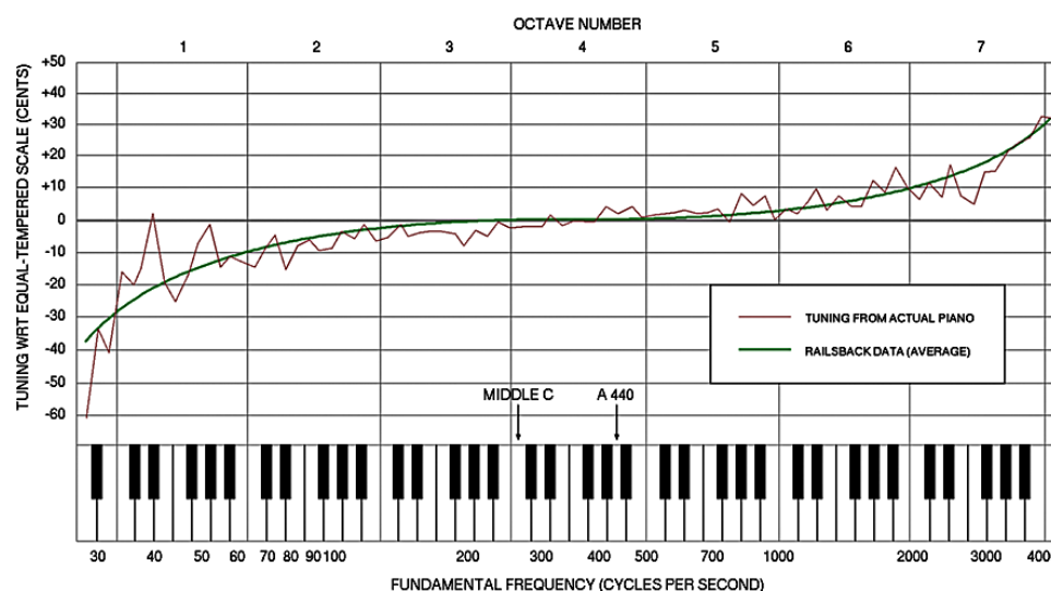
Figure 1 - Typical tuning curve of a piano (figure taken from [3]). The plot shows how much the fundamental frequency of each note deviates from the equal-tempered scale. The deviations are measured in cents , defined as 1/100 of a half-tone which corresponds to a frequency ratio of 2^{1/1200} \approx 1.0005778 .
