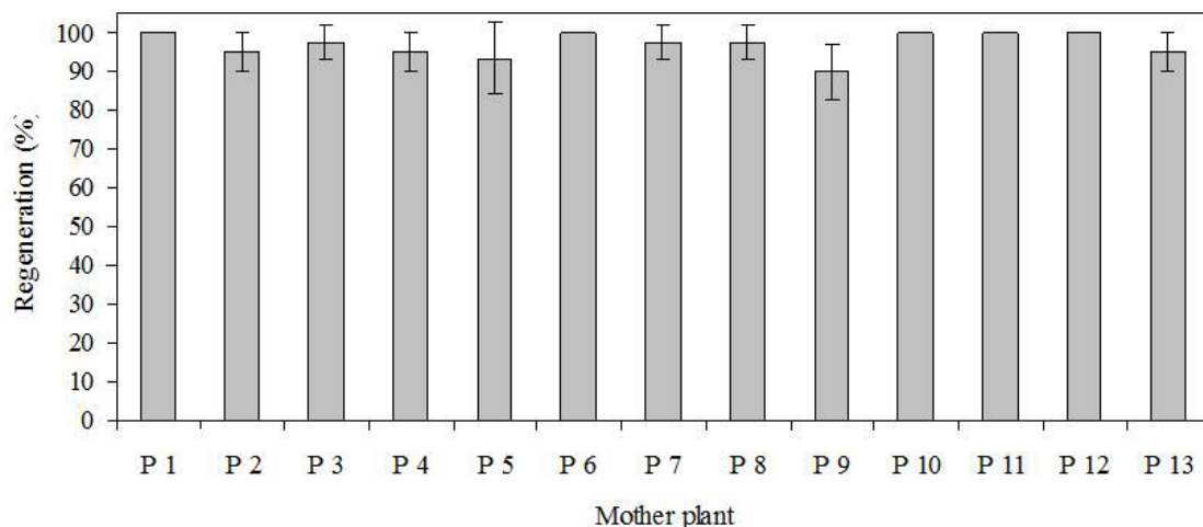
Figure 8 - Regeneration percentage of bacuri plants ( Platonia insignis Mart.) originating from the primary root of seeds of different mother plants. Source: CARVALHO, J.E.U. de; NASCIMENTO, W.M.O. do. (Unpublished data).
