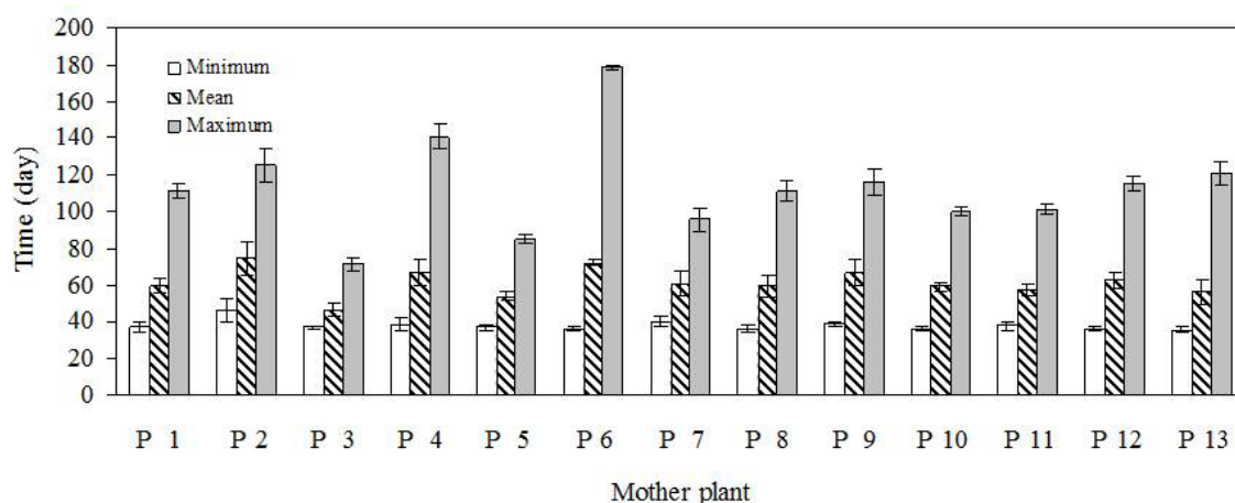
Figure 9 - Minimum, mean and maximum times required for the regeneration of bacuri plants ( Platonia insignis Mart.) from the primary root of seeds from different mother plants. Source: CARVALHO, J.E.U. de; NASCIMENTO, W.M.O. do. (Unpublished data).
