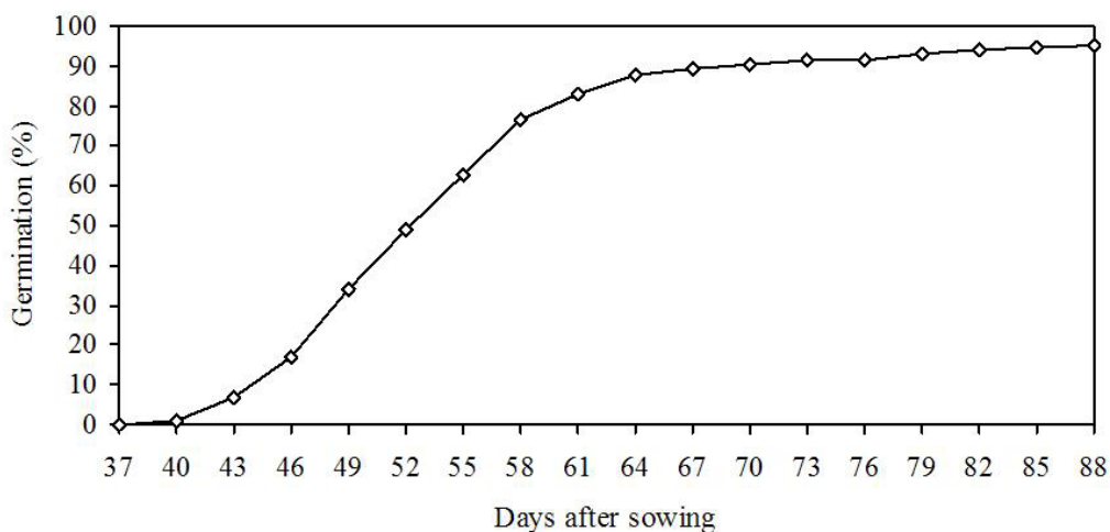
Figure 2 - Germination of Amazon açai ( Euterpe precatória Mart.) seeds as a function of time. Source: CARVALHO, J.E.U. de; NASCIMENTO, W.M.O. do. (Unpublished data).
