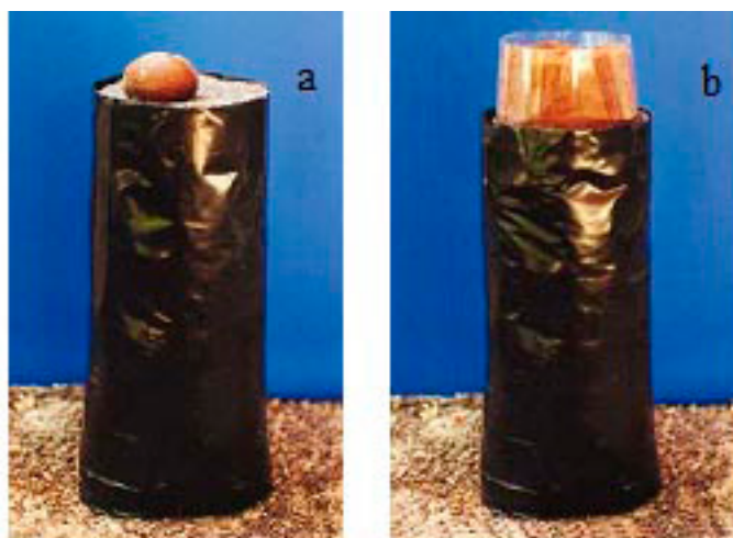
Figure 6 - Seed arrangement during sowing, with the root pole facing the center of the container (a) and seed protection with plastic cylinder filled with sawdust (b).
