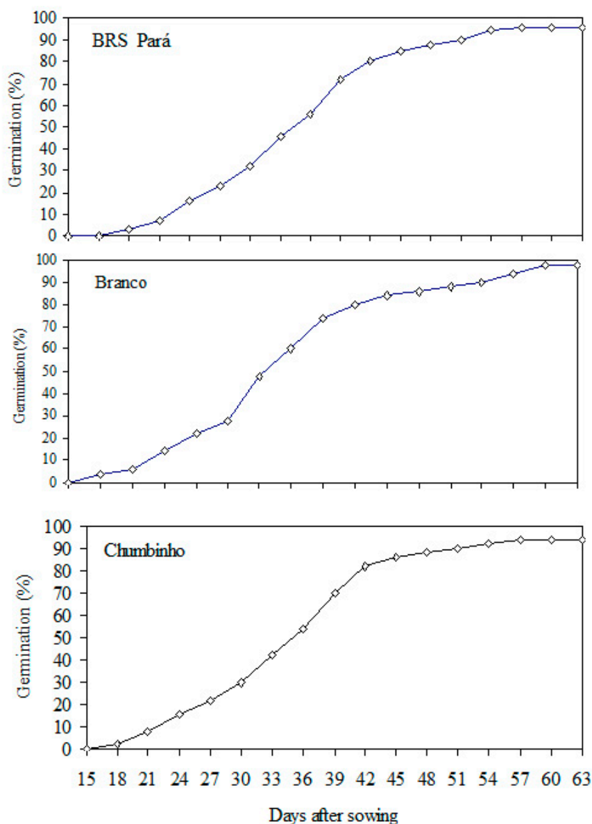
Figure 1 - Germination of açai ( Euterpe oleracea Mart.) seeds of BRS Pará, açai Branco and Chumbinho cultivars. Source: CARVALHO, J.E.U. de; NASCIMENTO, W.M.O. do. (Unpublished data).
