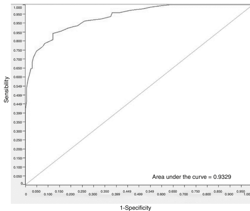
Fig. 3. ROC plot with the area under the curve for the test set of the E. coli model obtained with Random Forest.
