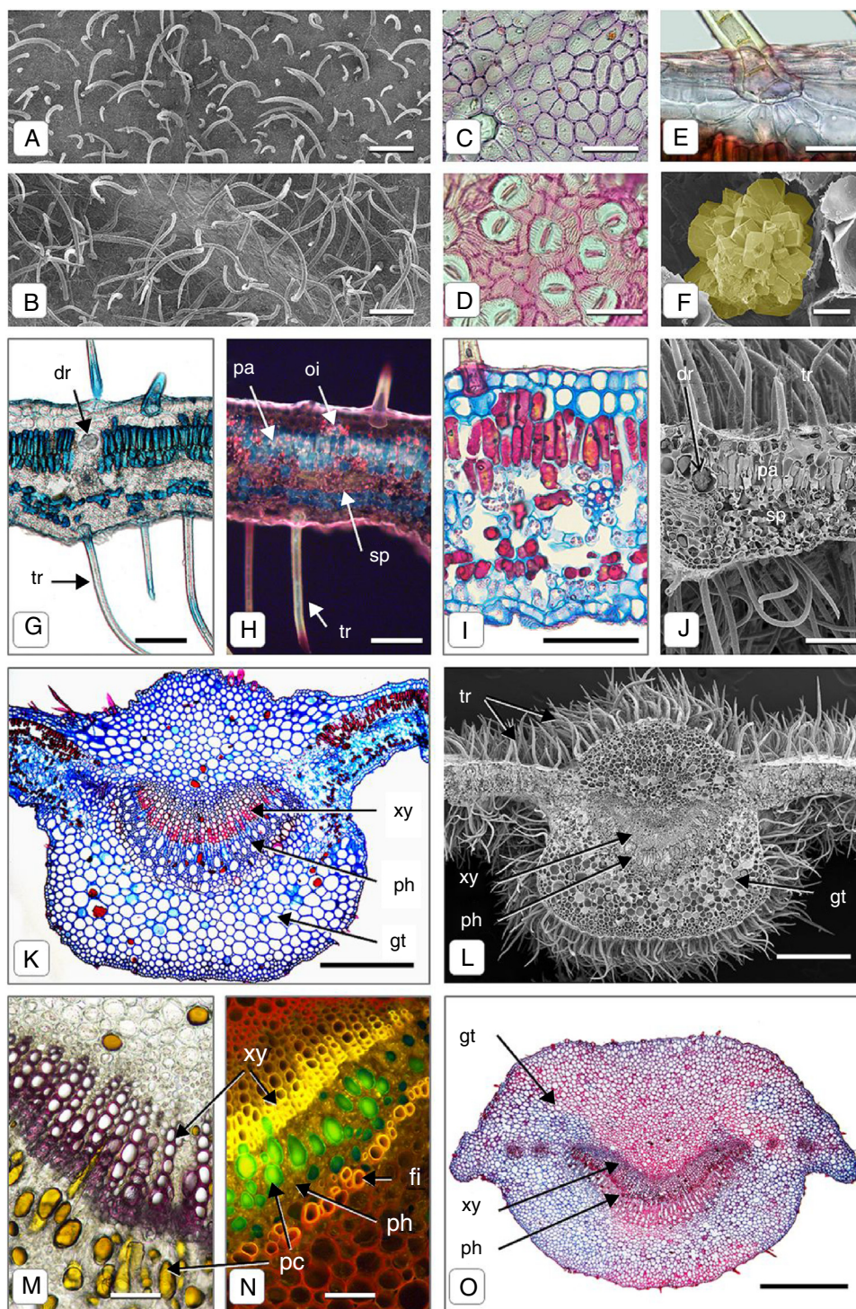
Fig. 1. Leaf anatomy of Fadogia agrestis [A, B, F, J, L: SEM images; C–E, G, I, K, M, O: normal light and H, N: fluorescent light microscopy; C, D, I, K, O: astra blue/basic fuchsin; F: colored SEM; G: stained in toluidine blue; M: phloroglucinol/HCl]. A, C: adaxial and B, D: abaxial leaf surface; E: base of a septate trichome; F: druse crystal in mesophyll; G–J: leaf blade in cross section showing phenolic contents, oil bodies and druse crystals in the mesophyll; K–N: leaf midrib in cross section; M, N: portions of vascular bundle showing xylem, phloem with several idioblasts containing phenolic contents, and medullary fibers; o: petiole in cross section. (dr, druse crystal; gt, ground tissue; fi, fibers; oi, oil bodies; pa, palisade tissue; pc, phenolic contents; ph, phloem; sp, spongy tissue; tr, trichome; xy, xylem). Bars: A, B = 200 \mu\text{m} ; C, D = 50 \mu\text{m} ; E = 20 \mu\text{m} ; F = 10 \mu\text{m} ; G–J, M, N = 100 \mu\text{m} ; K, L = 500 \mu\text{m} ; O = 1 mm.
