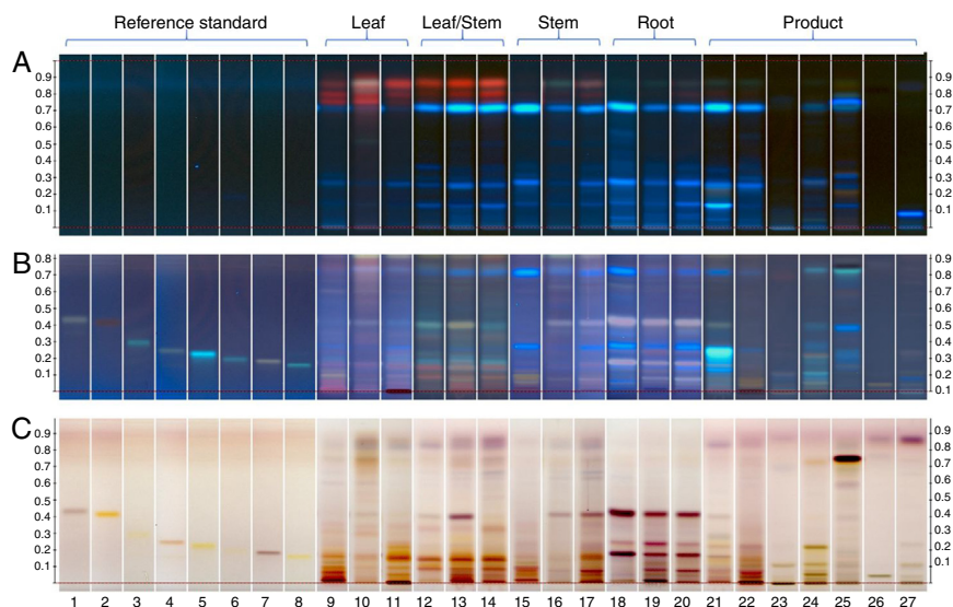
Fig. 5. HPTLC under UV 366 nm prior to derivatization (A), UV 366 nm after derivatization (B), and under white light after derivatization. Tracks 1–8: reference standards (1. 3- O - \alpha -L-Rhamnopyranosyl-(1 \rightarrow 2)- \alpha -L-arabinopyranosyl pomolic acid; 2. 2,4',6-Trihydroxy-4-methoxybenzophenone-2- O - \beta -D-glucoside; 3. Hyperoside; 4. Geniposidic acid; 5. Nicotiflorin; 6. Narcissin; 7. Randiasaponin IV; 8. Rutin); tracks 9–11: leaf samples (9. #13511; 10. #20086; 11. #20089); tracks 12–14: leaf/stem samples (12. #20102; 13. #20103; 14. #20104); tracks 15–17: stem samples (15. #13512; 16. #20087; 17. #20092); tracks 18–20: root samples (18. #1472; 19. #17094; 20. #18299); tracks 21–27: dietary supplement products claiming to contain Fadogia agrestis (21. #16838; 22. #19300; 23. #19303; 24. #19305; 25. #19307; 26. #19308; 27. #19309).
